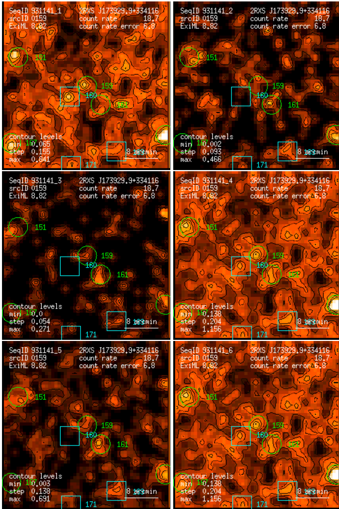
Figure 159: RASS 931141: detection 0159: band rate images, Gaussian filter: (1) PSPC channels 11 – 41, (2) 52 – 90, (3) 91 – 201, (4) 11 – 235, (5) 52 – 201, (6) 11 – 201. Broad band rates in counts/ks. Band rate contour levels in counts/ks/arcmin 2 .
