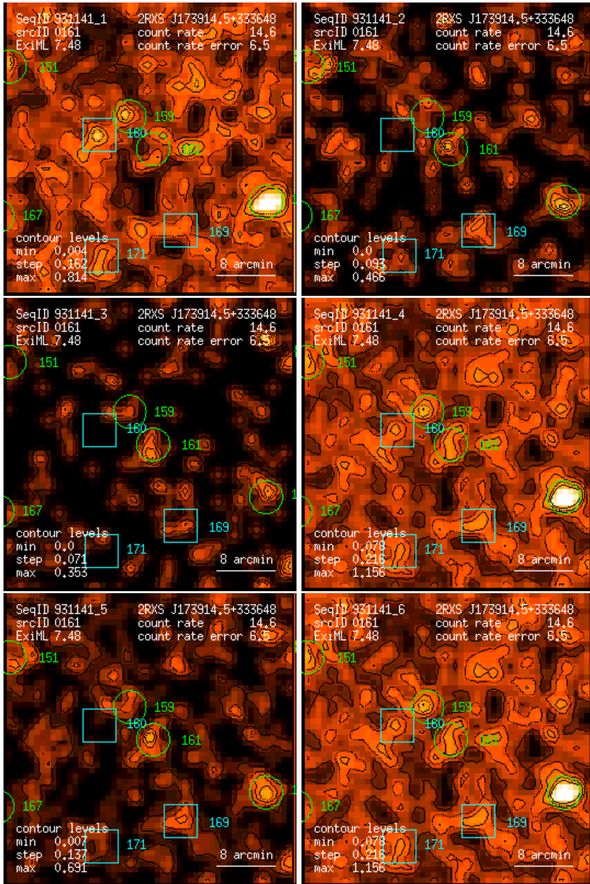
Figure 161: RASS 931141: detection 0161: band rate images, Gaussian filter: (1) PSPC channels 11 – 41, (2) 52 – 90, (3) 91 – 201, (4) 11 – 235, (5) 52 – 201, (6) 11 – 201. Broad band rates in counts/ks. Band rate contour levels in counts/ks/arcmin 2 .
