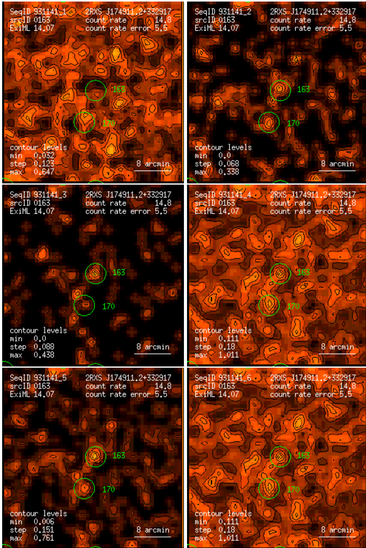
Figure 163: RASS 931141: detection 0163: band rate images, Gaussian filter: (1) PSPC channels 11 – 41, (2) 52 – 90, (3) 91 – 201, (4) 11 – 235, (5) 52 – 201, (6) 11 – 201. Broad band rates in counts/ks. Band rate contour levels in counts/ks/arcmin 2 .
