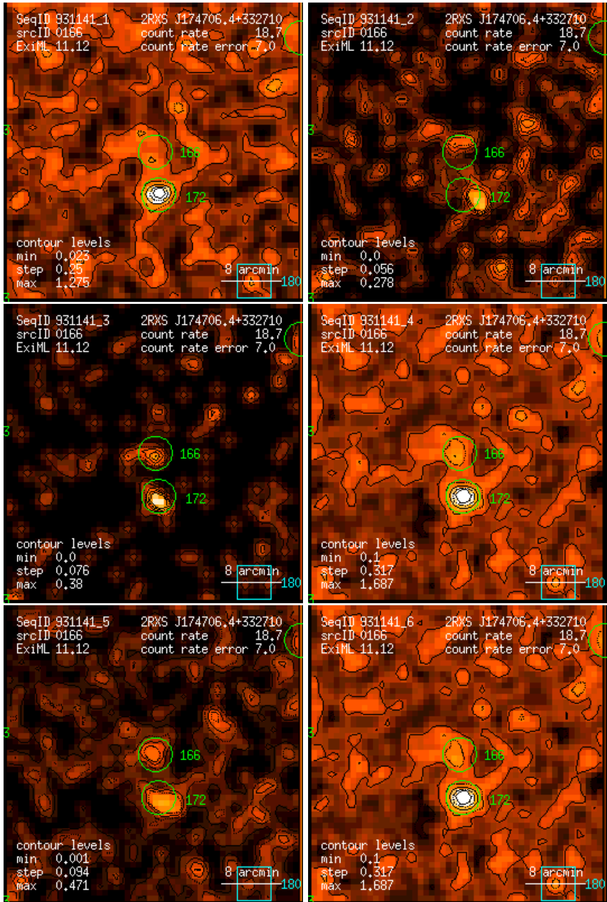
Figure 166: RASS 931141: detection 0166: band rate images, Gaussian filter: (1) PSPC channels 11 – 41, (2) 52 – 90, (3) 91 – 201, (4) 11 – 235, (5) 52 – 201, (6) 11 – 201. Broad band rates in counts/ks. Band rate contour levels in counts/ks/arcmin 2 .
