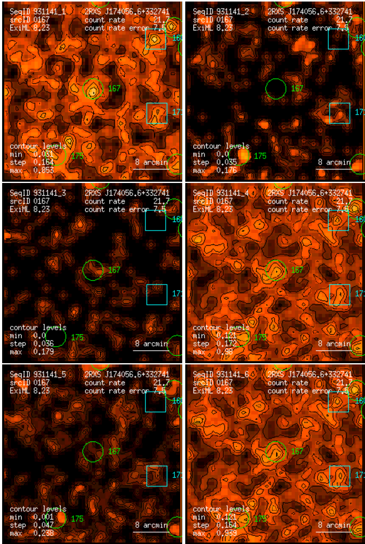
Figure 167: RASS 931141: detection 0167: band rate images, Gaussian filter: (1) PSPC channels 11 – 41, (2) 52 – 90, (3) 91 – 201, (4) 11 – 235, (5) 52 – 201, (6) 11 – 201. Broad band rates in counts/ks. Band rate contour levels in counts/ks/arcmin 2 .
