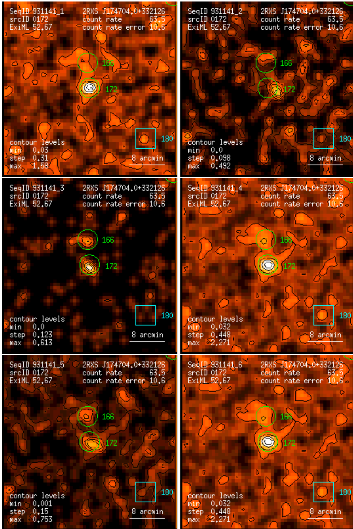
Figure 172: RASS 931141: detection 0172: band rate images, Gaussian filter: (1) PSPC channels 11 – 41, (2) 52 – 90, (3) 91 – 201, (4) 11 – 235, (5) 52 – 201, (6) 11 – 201. Broad band rates in counts/ks. Band rate contour levels in counts/ks/arcmin 2 .
