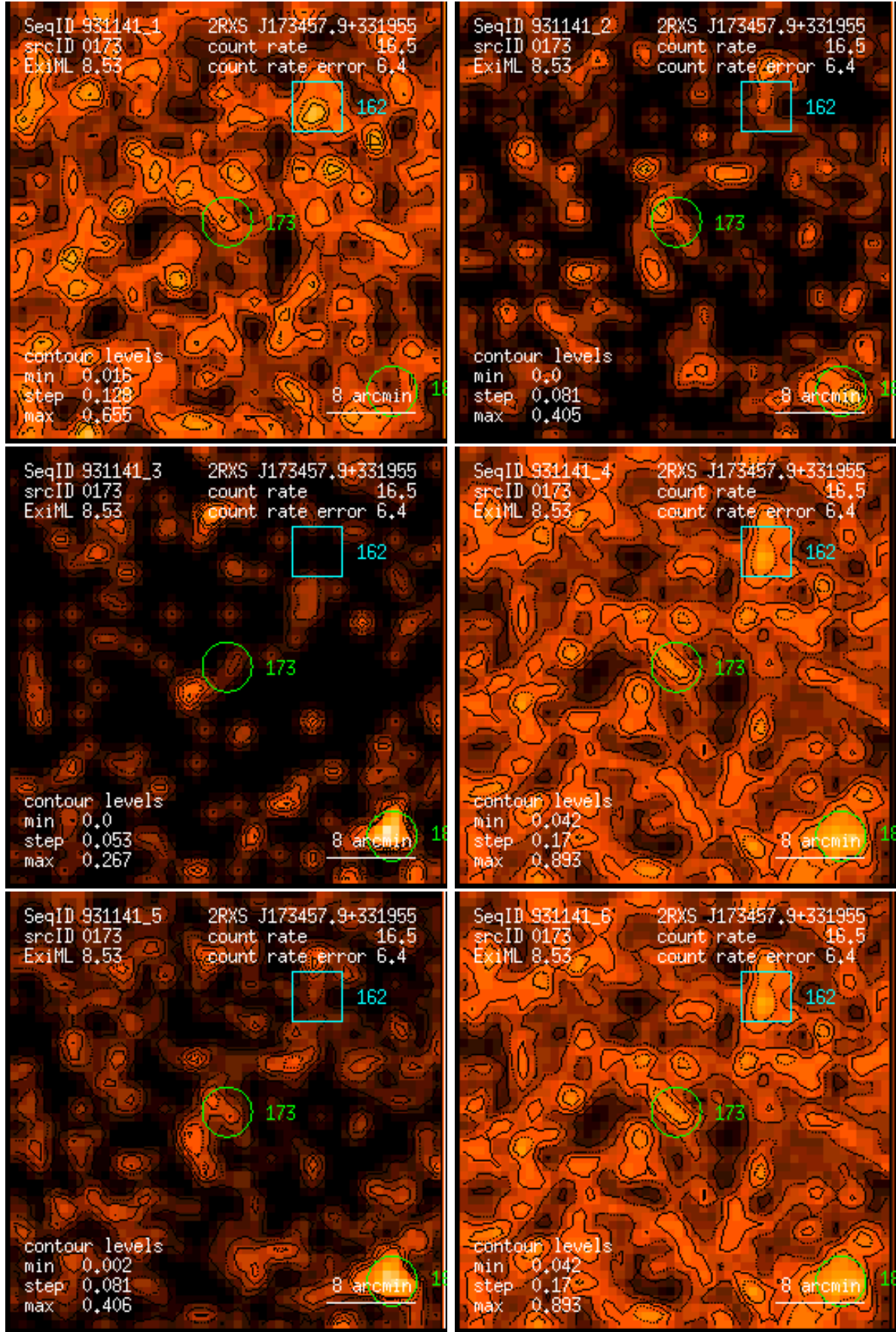
Figure 173: RASS 931141: detection 0173: band rate images, Gaussian filter: (1) PSPC channels 11 – 41, (2) 52 – 90, (3) 91 – 201, (4) 11 – 235, (5) 52 – 201, (6) 11 – 201. Broad band rates in counts/ks. Band rate contour levels in counts/ks/arcmin 2 .
