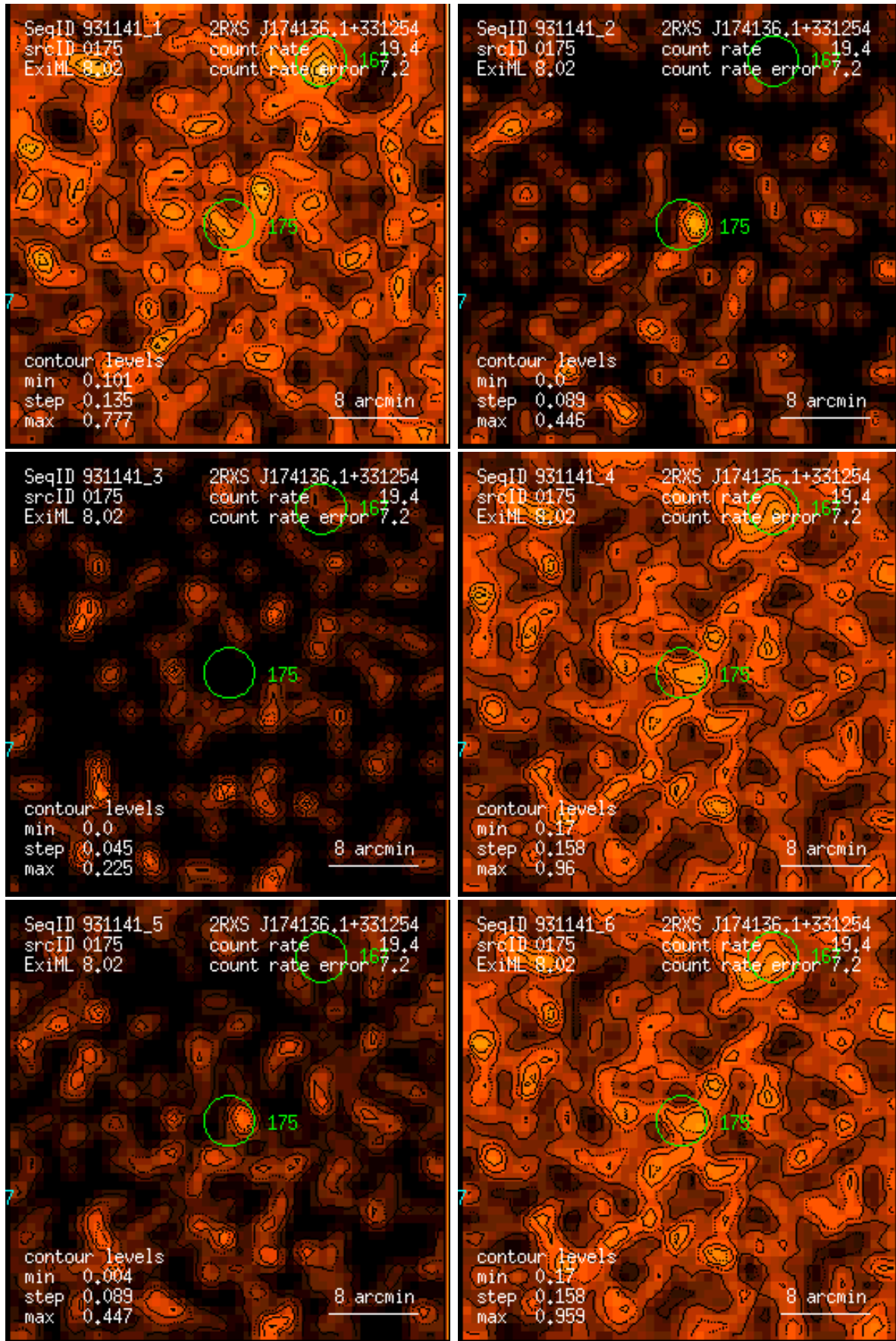
Figure 175: RASS 931141: detection 0175: band rate images, Gaussian filter: (1) PSPC channels 11 – 41, (2) 52 – 90, (3) 91 – 201, (4) 11 – 235, (5) 52 – 201, (6) 11 – 201. Broad band rates in counts/ks. Band rate contour levels in counts/ks/arcmin 2 .
