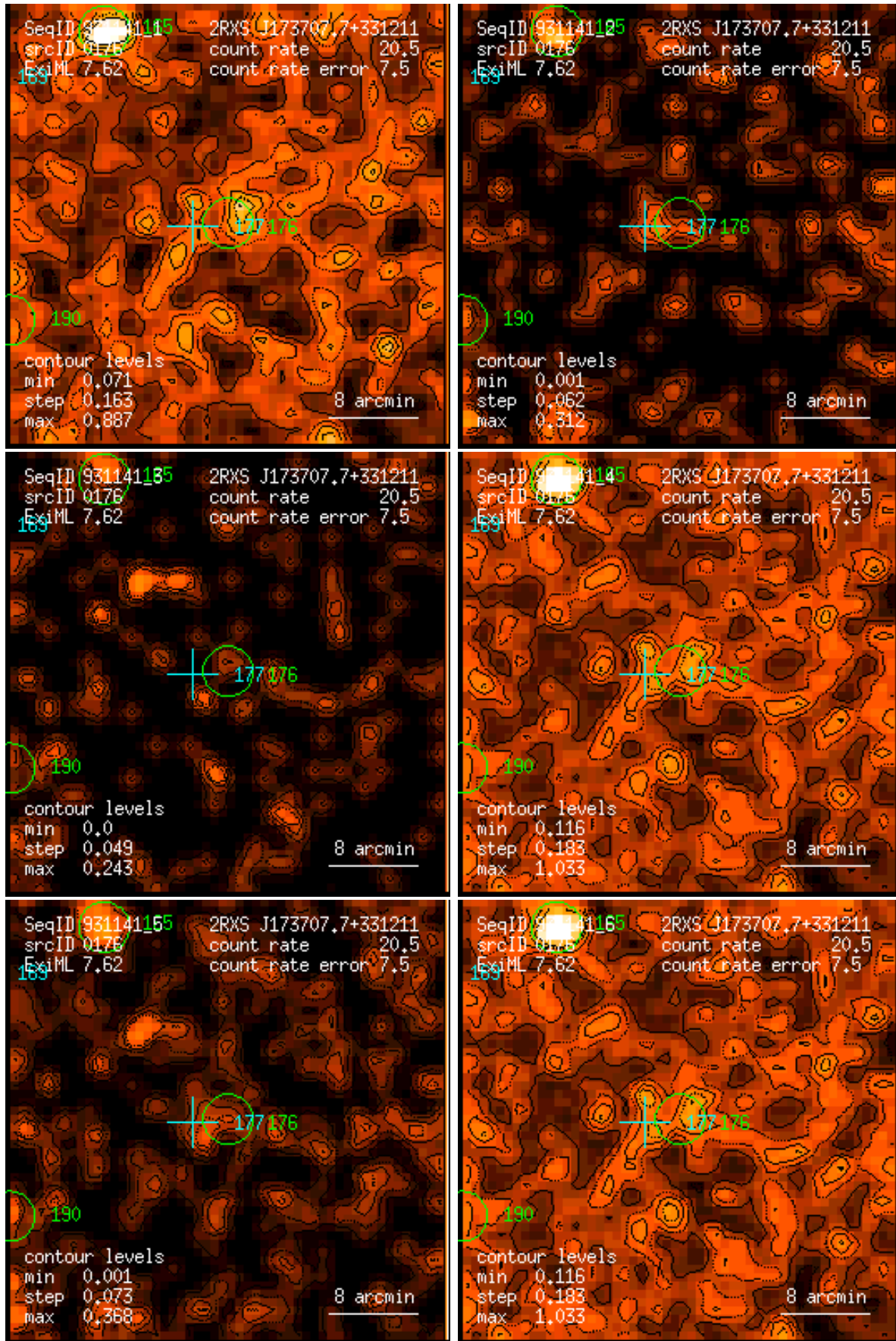
Figure 176: RASS 931141: detection 0176: band rate images, Gaussian filter: (1) PSPC channels 11 – 41, (2) 52 – 90, (3) 91 – 201, (4) 11 – 235, (5) 52 – 201, (6) 11 – 201. Broad band rates in counts/ks. Band rate contour levels in counts/ks/arcmin 2 .
