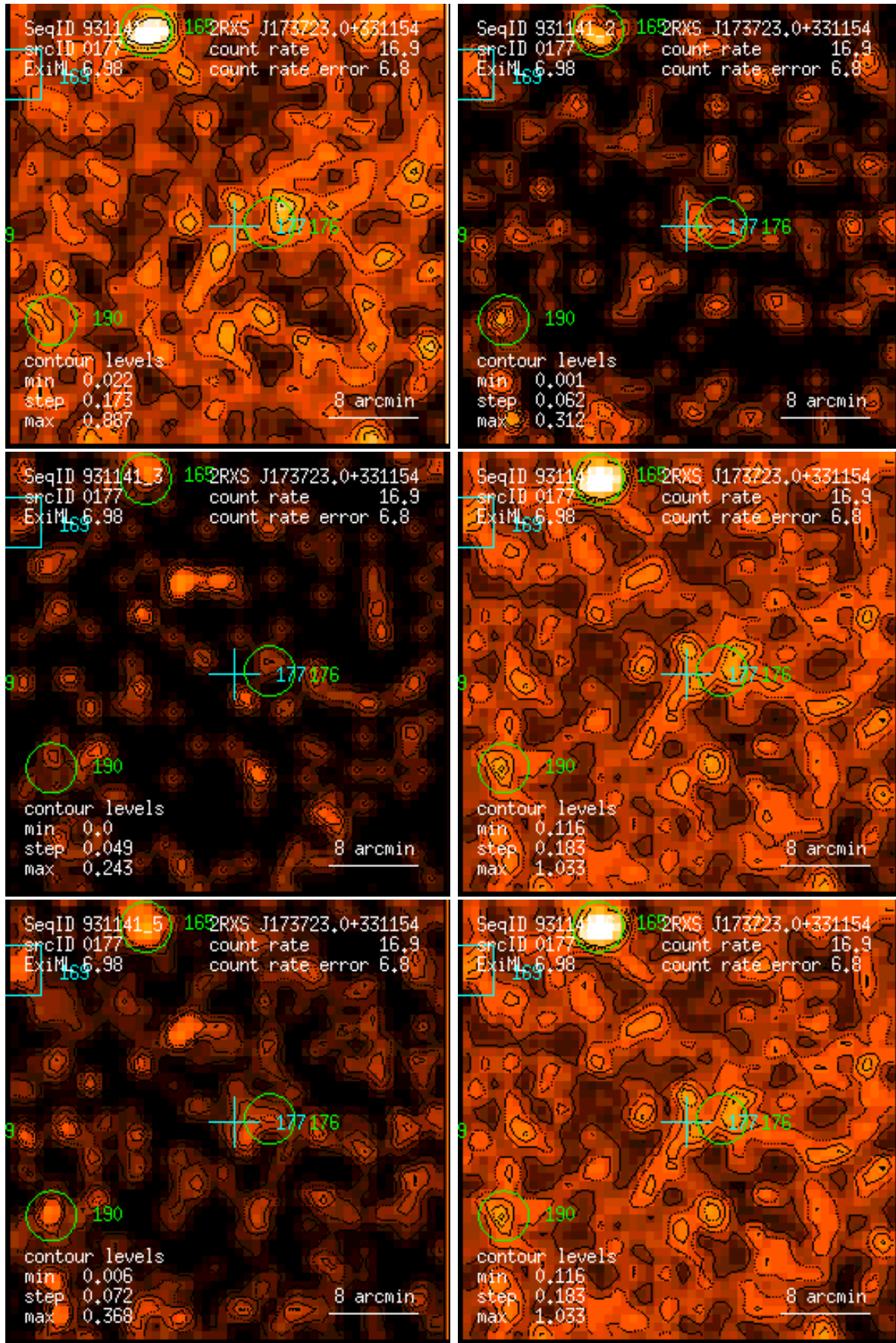
Figure 177: RASS 931141: detection 0177: band rate images, Gaussian filter: (1) PSPC channels 11 – 41, (2) 52 – 90, (3) 91 – 201, (4) 11 – 235, (5) 52 – 201, (6) 11 – 201. Broad band rates in counts/ks. Band rate contour levels in counts/ks/arcmin 2 .
