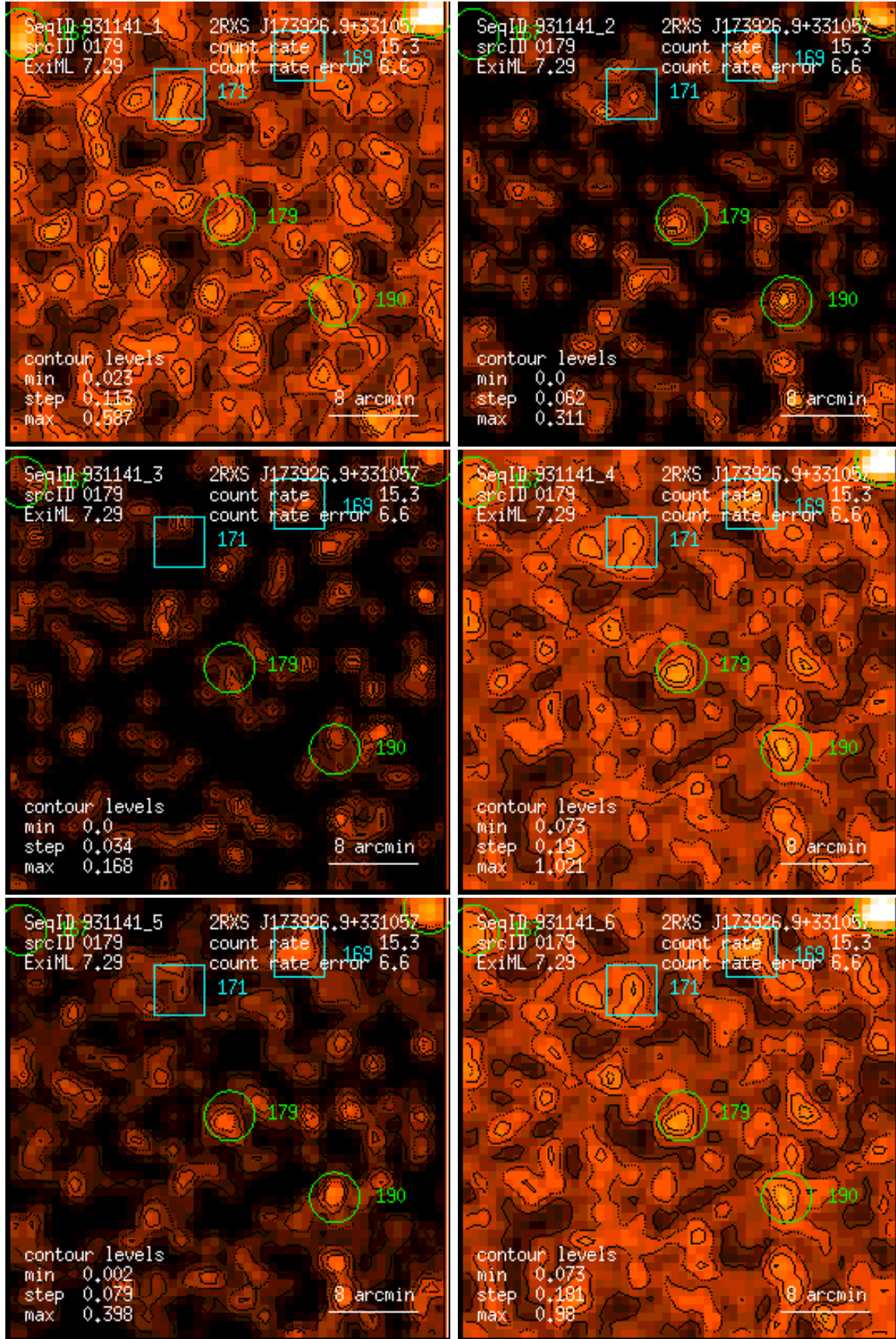
Figure 179: RASS 931141: detection 0179: band rate images, Gaussian filter: (1) PSPC channels 11 – 41, (2) 52 – 90, (3) 91 – 201, (4) 11 – 235, (5) 52 – 201, (6) 11 – 201. Broad band rates in counts/ks. Band rate contour levels in counts/ks/arcmin 2 .
