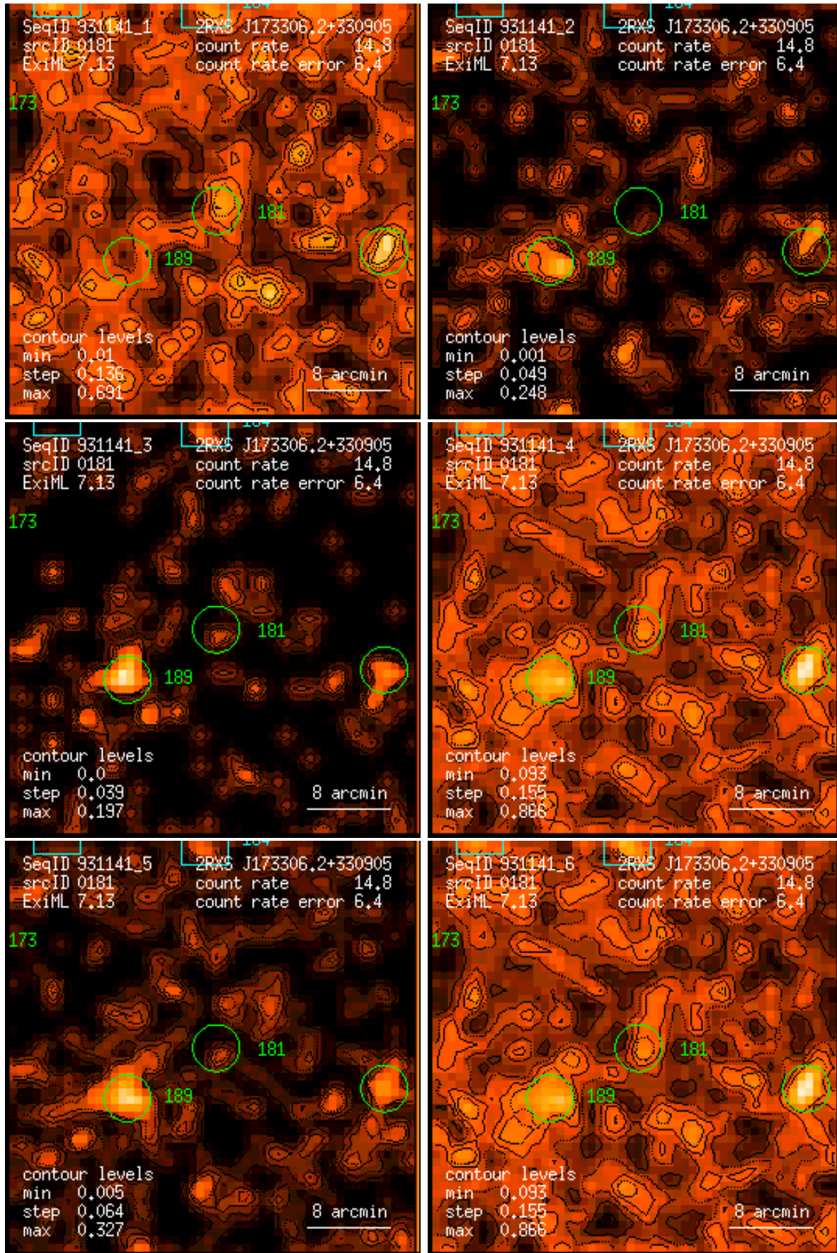
Figure 181: RASS 931141: detection 0181: band rate images, Gaussian filter: (1) PSPC channels 11 – 41, (2) 52 – 90, (3) 91 – 201, (4) 11 – 235, (5) 52 – 201, (6) 11 – 201. Broad band rates in counts/ks. Band rate contour levels in counts/ks/arcmin 2 .
