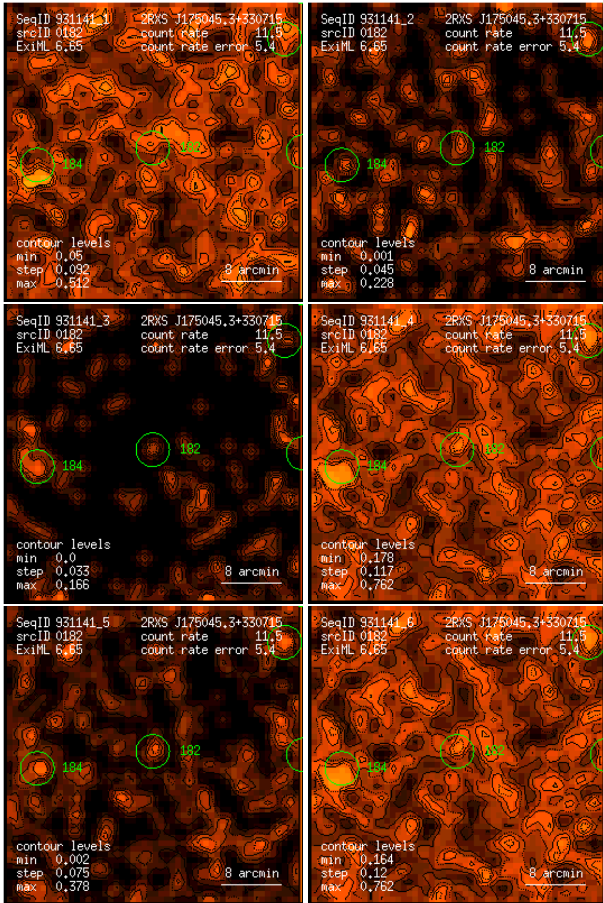
Figure 182: RASS 931141: detection 0182: band rate images, Gaussian filter: (1) PSPC channels 11 – 41, (2) 52 – 90, (3) 91 – 201, (4) 11 – 235, (5) 52 – 201, (6) 11 – 201. Broad band rates in counts/ks. Band rate contour levels in counts/ks/arcmin 2 .
