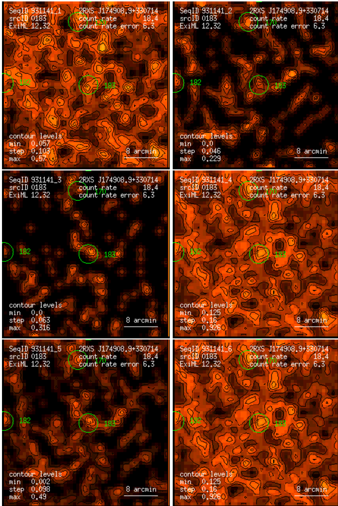
Figure 183: RASS 931141: detection 0183: band rate images, Gaussian filter: (1) PSPC channels 11 – 41, (2) 52 – 90, (3) 91 – 201, (4) 11 – 235, (5) 52 – 201, (6) 11 – 201. Broad band rates in counts/ks. Band rate contour levels in counts/ks/arcmin 2 .
