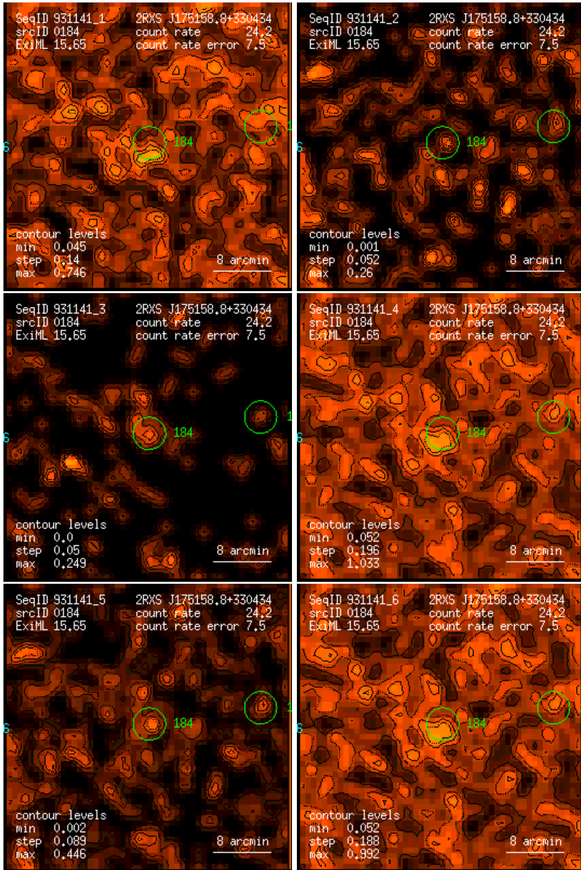
Figure 184: RASS 931141: detection 0184: band rate images, Gaussian filter: (1) PSPC channels 11 – 41, (2) 52 – 90, (3) 91 – 201, (4) 11 – 235, (5) 52 – 201, (6) 11 – 201. Broad band rates in counts/ks. Band rate contour levels in counts/ks/arcmin 2 .
