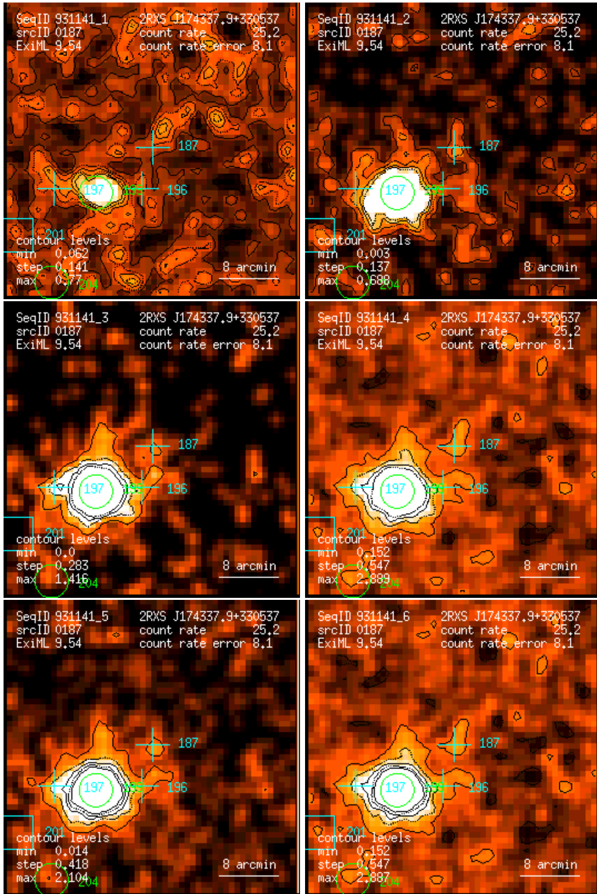
Figure 187: RASS 931141: detection 0187: band rate images, Gaussian filter: (1) PSPC channels 11 – 41, (2) 52 – 90, (3) 91 – 201, (4) 11 – 235, (5) 52 – 201, (6) 11 – 201. Broad band rates in counts/ks. Band rate contour levels in counts/ks/arcmin 2 .
