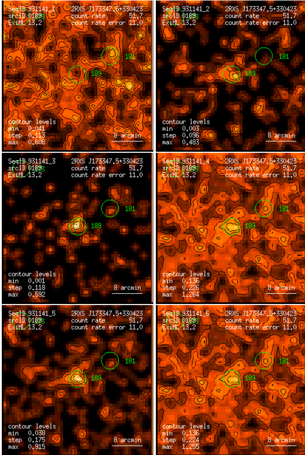
Figure 189: RASS 931141: detection 0189: band rate images, Gaussian filter: (1) PSPC channels 11 – 41, (2) 52 – 90, (3) 91 – 201, (4) 11 – 235, (5) 52 – 201, (6) 11 – 201. Broad band rates in counts/ks. Band rate contour levels in counts/ks/arcmin 2 .
