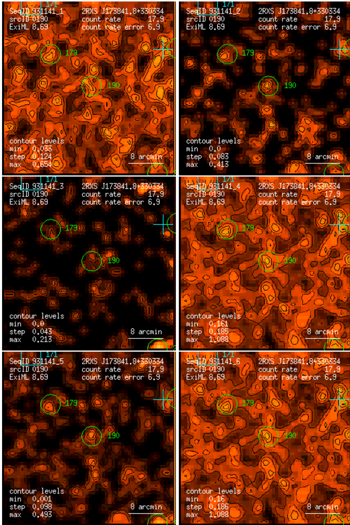
Figure 190: RASS 931141: detection 0190: band rate images, Gaussian filter: (1) PSPC channels 11 – 41, (2) 52 – 90, (3) 91 – 201, (4) 11 – 235, (5) 52 – 201, (6) 11 – 201. Broad band rates in counts/ks. Band rate contour levels in counts/ks/arcmin 2 .
