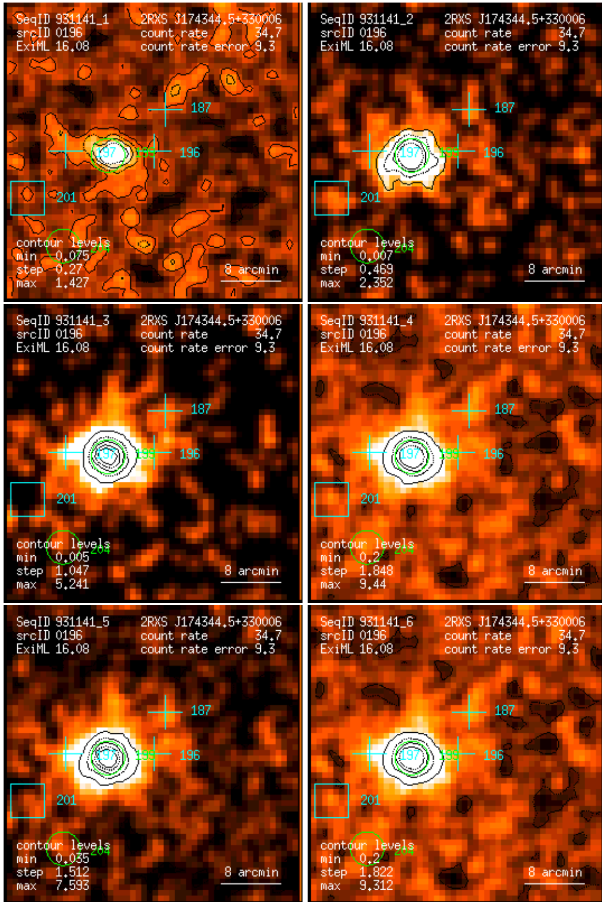
Figure 196: RASS 931141: detection 0196: band rate images, Gaussian filter: (1) PSPC channels 11 – 41, (2) 52 – 90, (3) 91 – 201, (4) 11 – 235, (5) 52 – 201, (6) 11 – 201. Broad band rates in counts/ks. Band rate contour levels in counts/ks/arcmin 2 .
