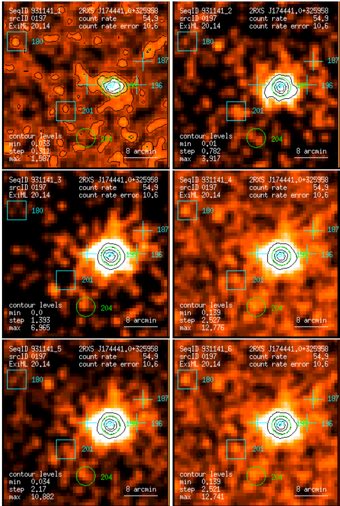
Figure 197: RASS 931141: detection 0197: band rate images, Gaussian filter: (1) PSPC channels 11 – 41, (2) 52 – 90, (3) 91 – 201, (4) 11 – 235, (5) 52 – 201, (6) 11 – 201. Broad band rates in counts/ks. Band rate contour levels in counts/ks/arcmin 2 .
