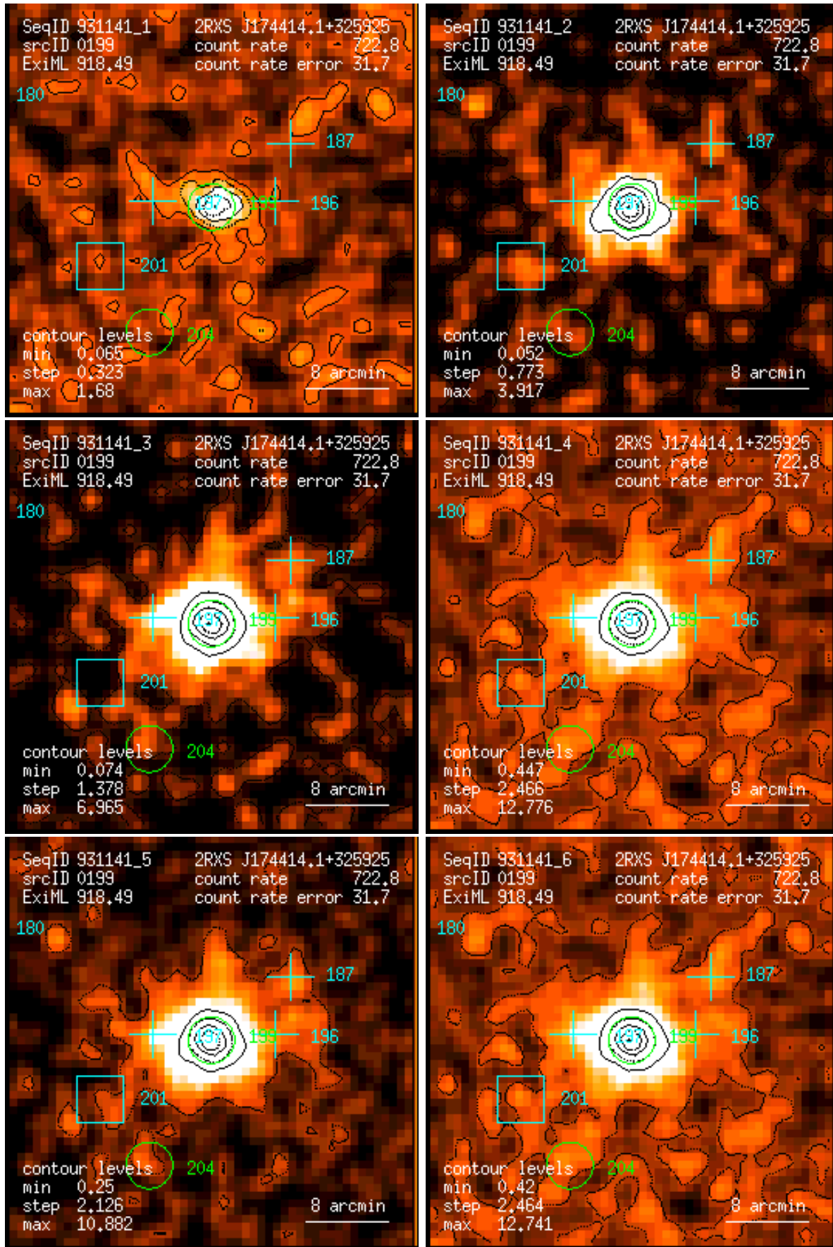
Figure 199: RASS 931141: detection 0199: band rate images, Gaussian filter: (1) PSPC channels 11 – 41, (2) 52 – 90, (3) 91 – 201, (4) 11 – 235, (5) 52 – 201, (6) 11 – 201. Broad band rates in counts/ks. Band rate contour levels in counts/ks/arcmin 2 .
