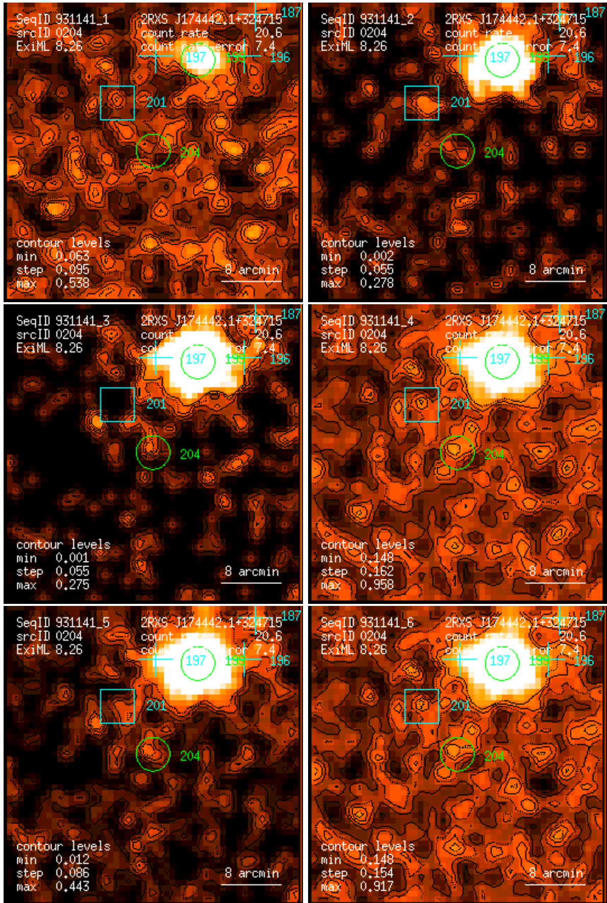
Figure 204: RASS 931141: detection 0204: band rate images, Gaussian filter: (1) PSPC channels 11 – 41, (2) 52 – 90, (3) 91 – 201, (4) 11 – 235, (5) 52 – 201, (6) 11 – 201. Broad band rates in counts/ks. Band rate contour levels in counts/ks/arcmin 2 .
