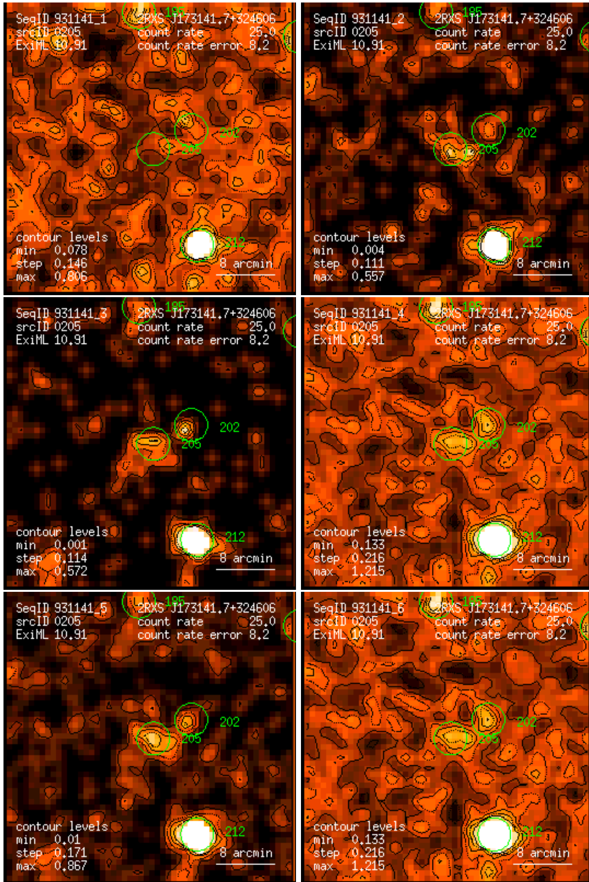
Figure 205: RASS 931141: detection 0205: band rate images, Gaussian filter: (1) PSPC channels 11 – 41, (2) 52 – 90, (3) 91 – 201, (4) 11 – 235, (5) 52 – 201, (6) 11 – 201. Broad band rates in counts/ks. Band rate contour levels in counts/ks/arcmin 2 .
