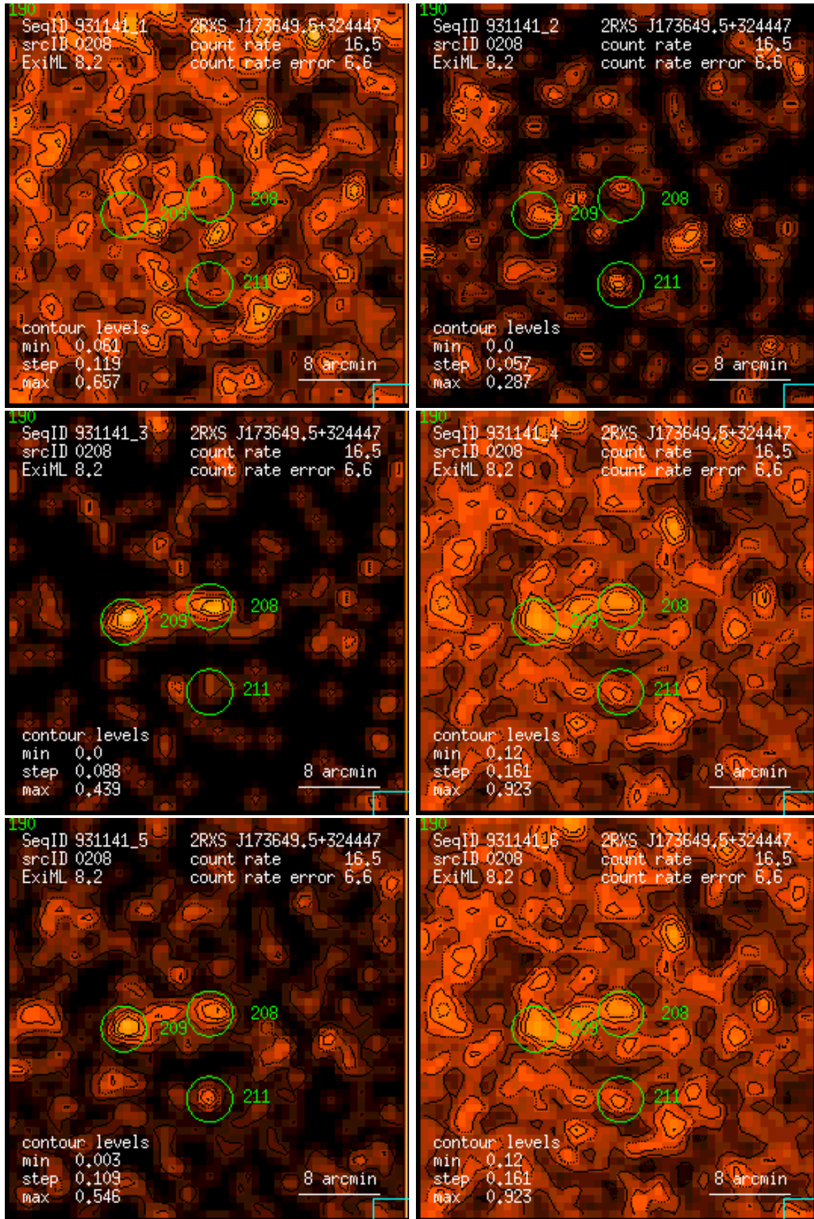
Figure 208: RASS 931141: detection 0208: band rate images, Gaussian filter: (1) PSPC channels 11 – 41, (2) 52 – 90, (3) 91 – 201, (4) 11 – 235, (5) 52 – 201, (6) 11 – 201. Broad band rates in counts/ks. Band rate contour levels in counts/ks/arcmin 2 .
