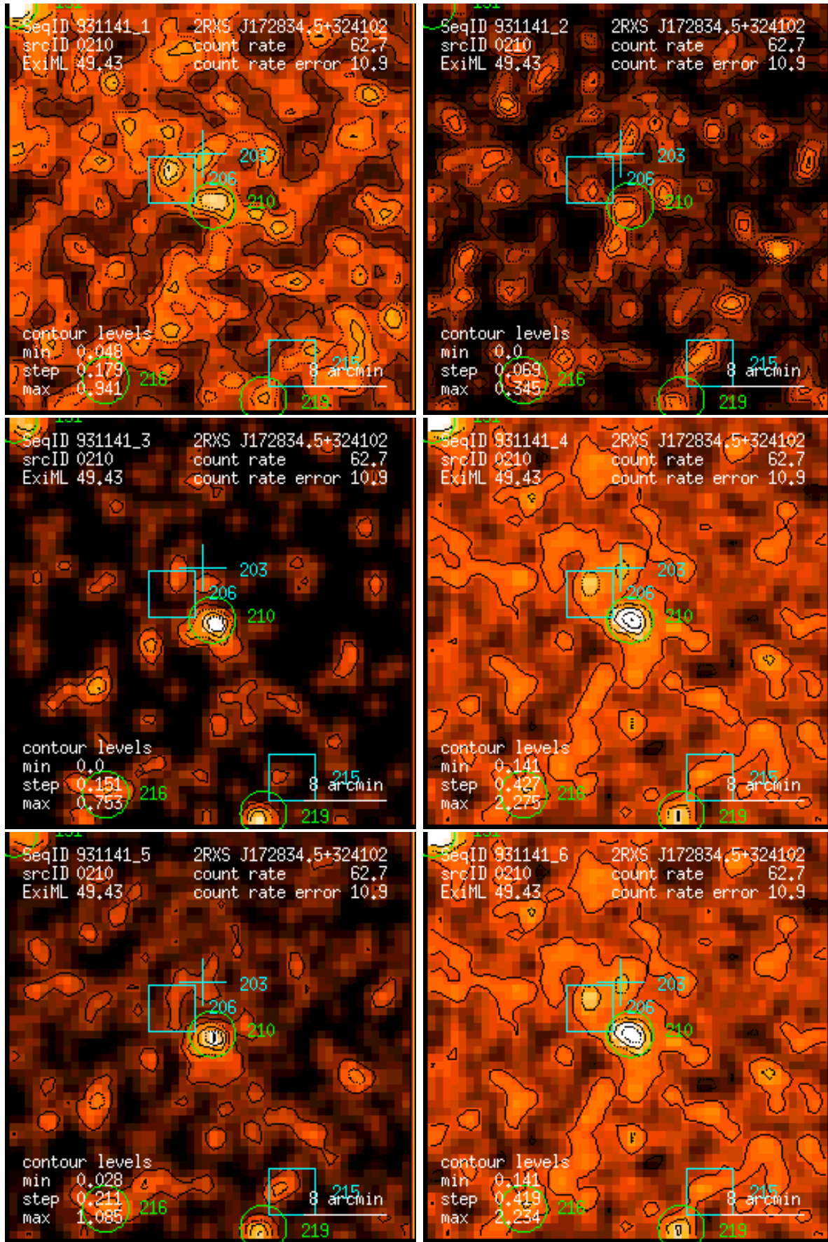
Figure 210: RASS 931141: detection 0210: band rate images, Gaussian filter: (1) PSPC channels 11 – 41, (2) 52 – 90, (3) 91 – 201, (4) 11 – 235, (5) 52 – 201, (6) 11 – 201. Broad band rates in counts/ks. Band rate contour levels in counts/ks/arcmin 2 .
