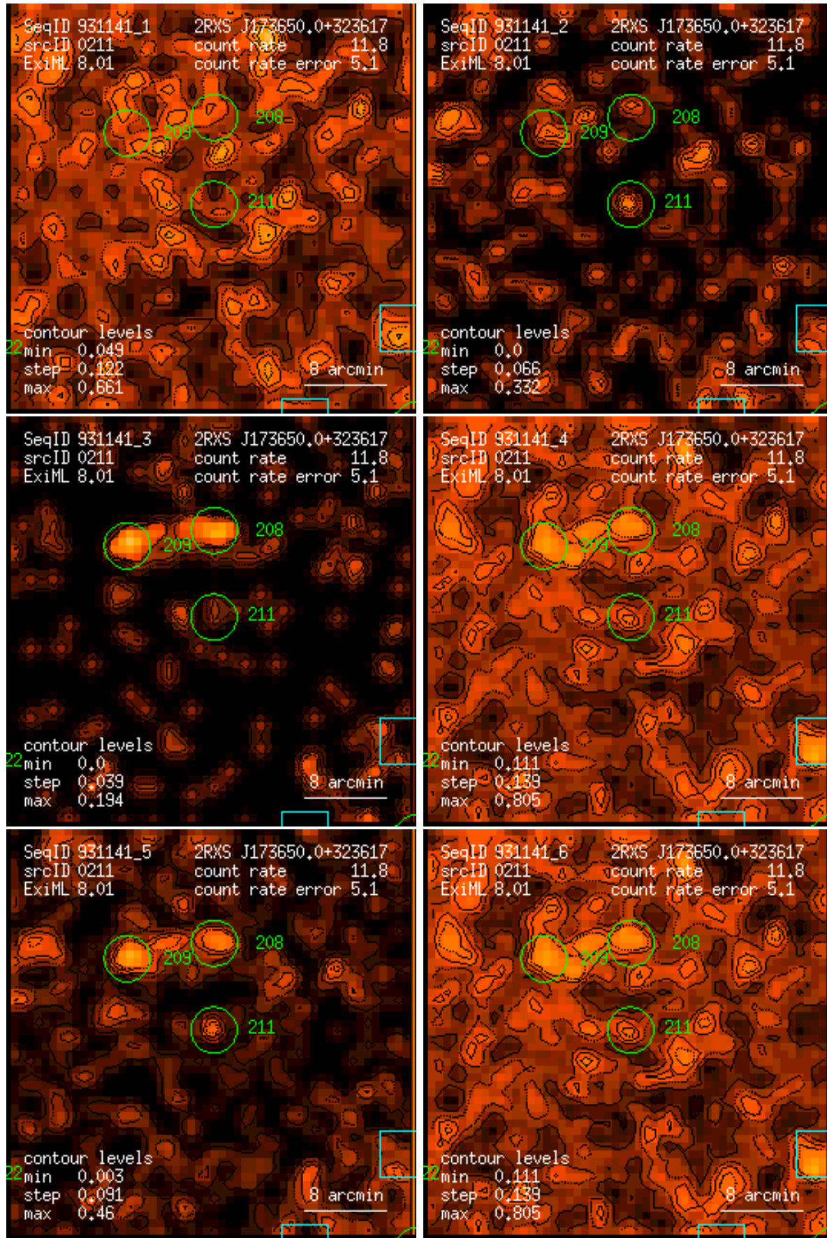
Figure 211: RASS 931141: detection 0211: band rate images, Gaussian filter: (1) PSPC channels 11 – 41, (2) 52 – 90, (3) 91 – 201, (4) 11 – 235, (5) 52 – 201, (6) 11 – 201. Broad band rates in counts/ks. Band rate contour levels in counts/ks/arcmin 2 .
