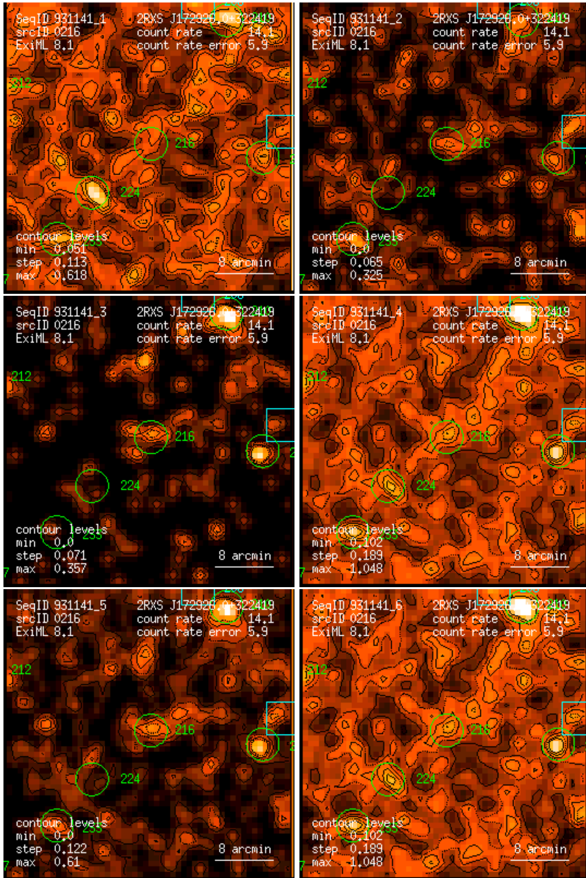
Figure 216: RASS 931141: detection 0216: band rate images, Gaussian filter: (1) PSPC channels 11 – 41, (2) 52 – 90, (3) 91 – 201, (4) 11 – 235, (5) 52 – 201, (6) 11 – 201. Broad band rates in counts/ks. Band rate contour levels in counts/ks/arcmin 2 .
