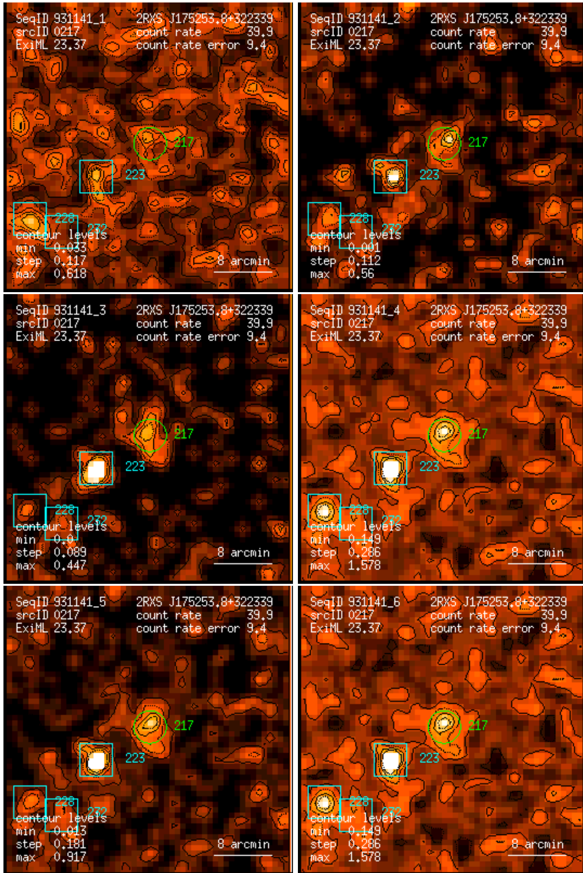
Figure 217: RASS 931141: detection 0217: band rate images, Gaussian filter: (1) PSPC channels 11 – 41, (2) 52 – 90, (3) 91 – 201, (4) 11 – 235, (5) 52 – 201, (6) 11 – 201. Broad band rates in counts/ks. Band rate contour levels in counts/ks/arcmin 2 .
