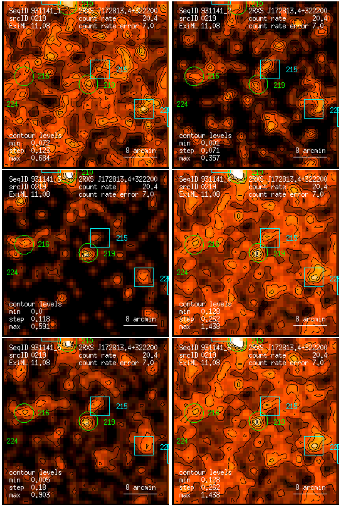
Figure 219: RASS 931141: detection 0219: band rate images, Gaussian filter: (1) PSPC channels 11 – 41, (2) 52 – 90, (3) 91 – 201, (4) 11 – 235, (5) 52 – 201, (6) 11 – 201. Broad band rates in counts/ks. Band rate contour levels in counts/ks/arcmin 2 .
