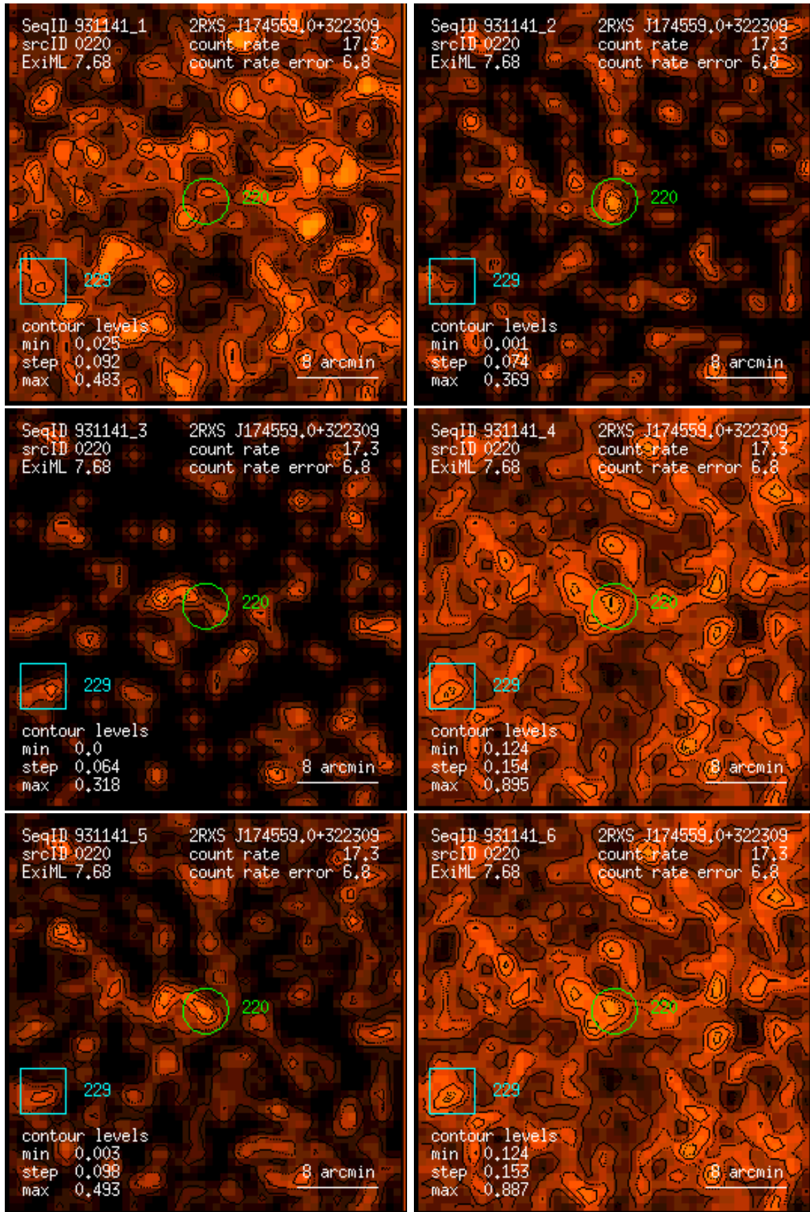
Figure 220: RASS 931141: detection 0220: band rate images, Gaussian filter: (1) PSPC channels 11 – 41, (2) 52 – 90, (3) 91 – 201, (4) 11 – 235, (5) 52 – 201, (6) 11 – 201. Broad band rates in counts/ks. Band rate contour levels in counts/ks/arcmin 2 .
