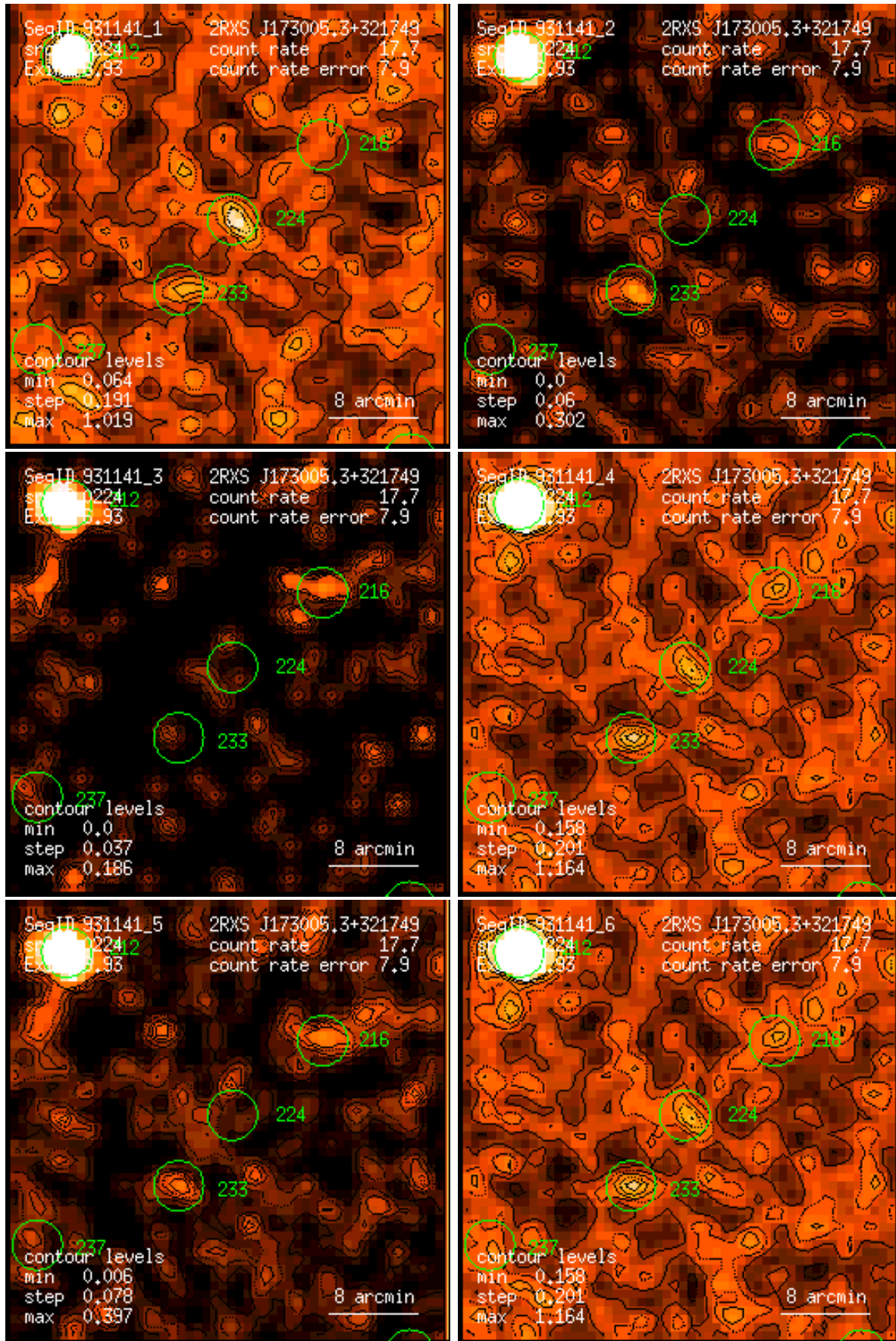
Figure 224: RASS 931141: detection 0224: band rate images, Gaussian filter: (1) PSPC channels 11 – 41, (2) 52 – 90, (3) 91 – 201, (4) 11 – 235, (5) 52 – 201, (6) 11 – 201. Broad band rates in counts/ks. Band rate contour levels in counts/ks/arcmin 2 .
