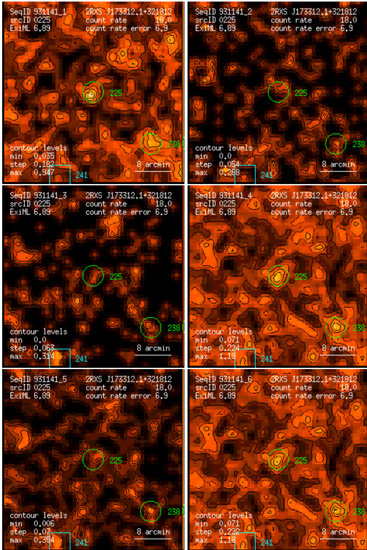
Figure 225: RASS 931141: detection 0225: band rate images, Gaussian filter: (1) PSPC channels 11 – 41, (2) 52 – 90, (3) 91 – 201, (4) 11 – 235, (5) 52 – 201, (6) 11 – 201. Broad band rates in counts/ks. Band rate contour levels in counts/ks/arcmin 2 .
