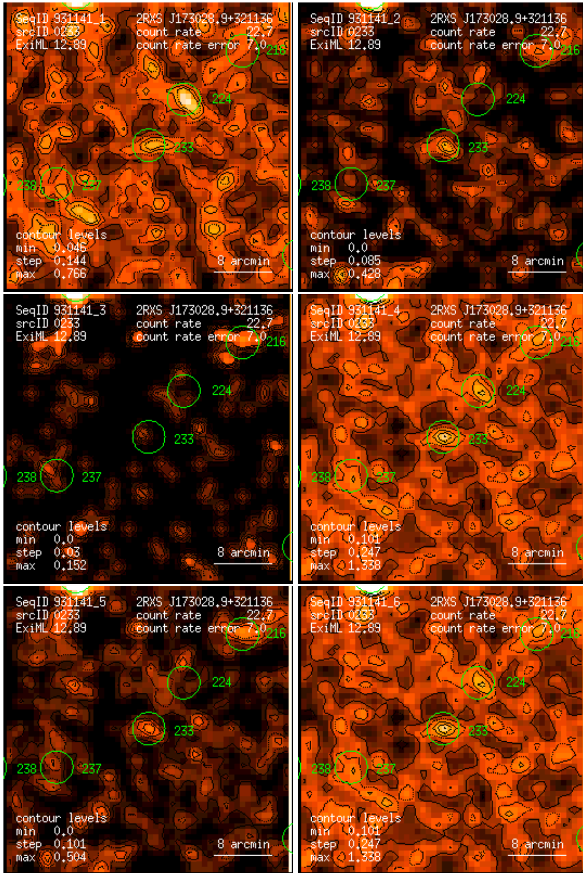
Figure 233: RASS 931141: detection 0233: band rate images, Gaussian filter: (1) PSPC channels 11 – 41, (2) 52 – 90, (3) 91 – 201, (4) 11 – 235, (5) 52 – 201, (6) 11 – 201. Broad band rates in counts/ks. Band rate contour levels in counts/ks/arcmin 2 .
