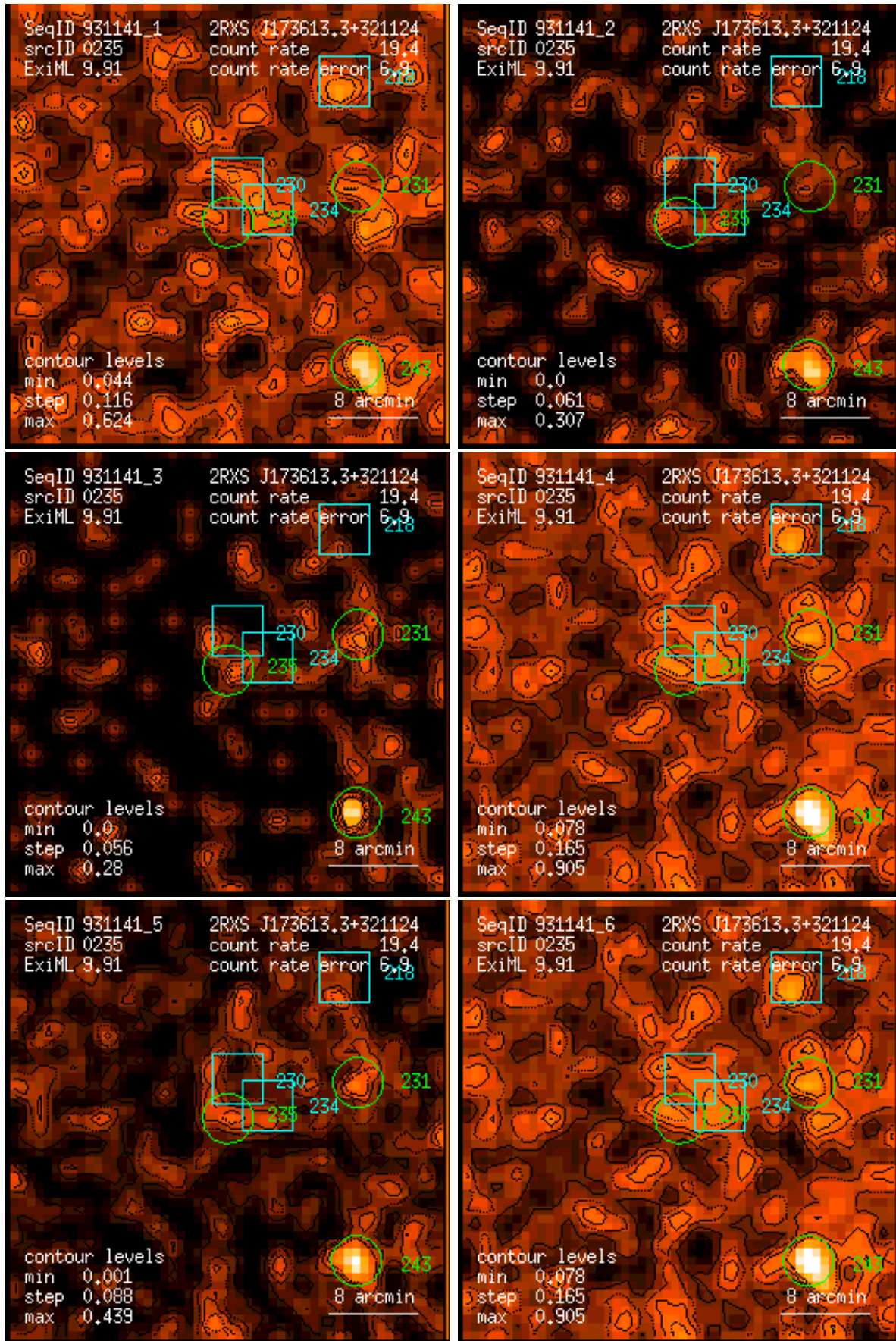
Figure 235: RASS 931141: detection 0235: band rate images, Gaussian filter: (1) PSPC channels 11 – 41, (2) 52 – 90, (3) 91 – 201, (4) 11 – 235, (5) 52 – 201, (6) 11 – 201. Broad band rates in counts/ks. Band rate contour levels in counts/ks/arcmin 2 .
