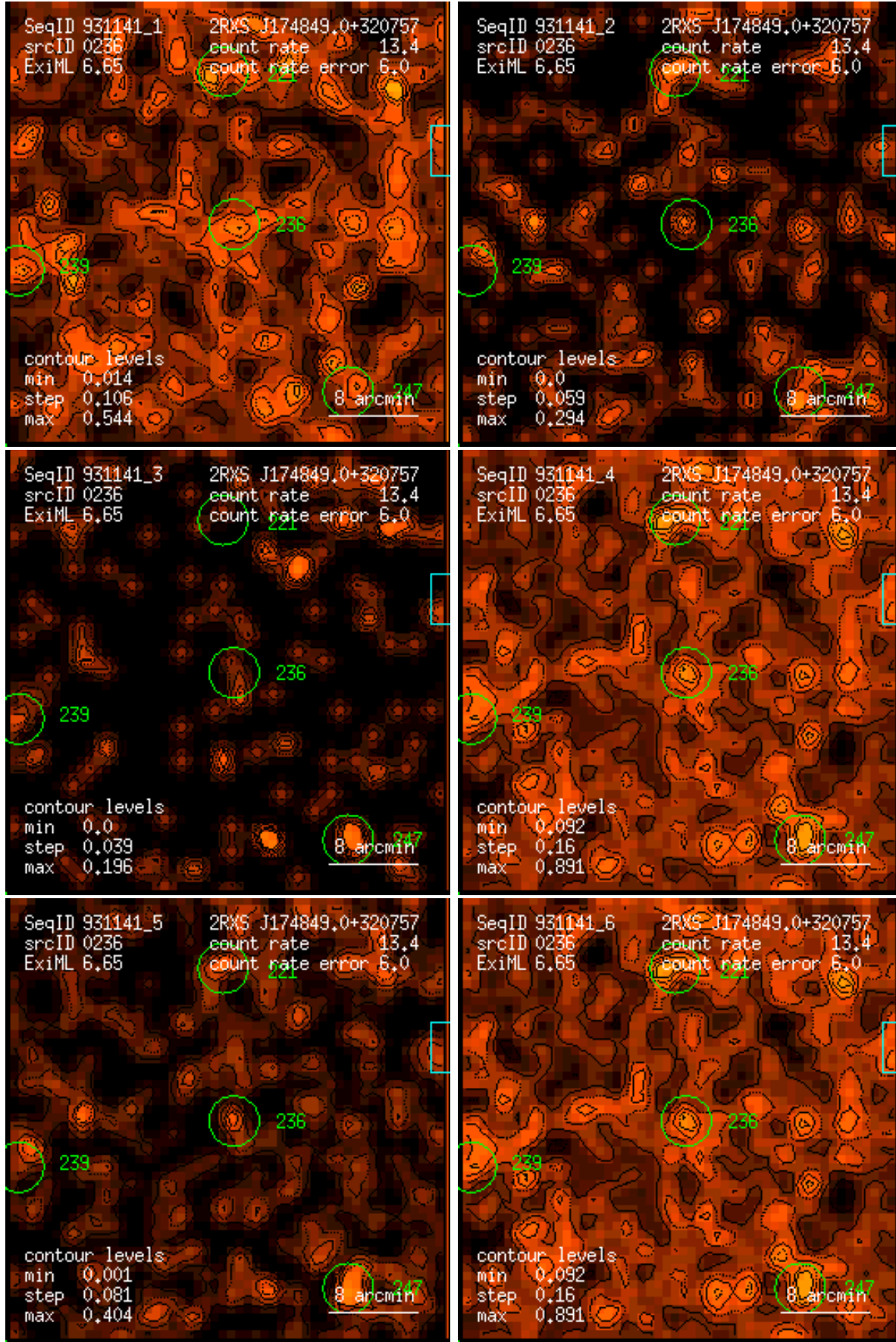
Figure 236: RASS 931141: detection 0236: band rate images, Gaussian filter: (1) PSPC channels 11 – 41, (2) 52 – 90, (3) 91 – 201, (4) 11 – 235, (5) 52 – 201, (6) 11 – 201. Broad band rates in counts/ks. Band rate contour levels in counts/ks/arcmin 2 .
