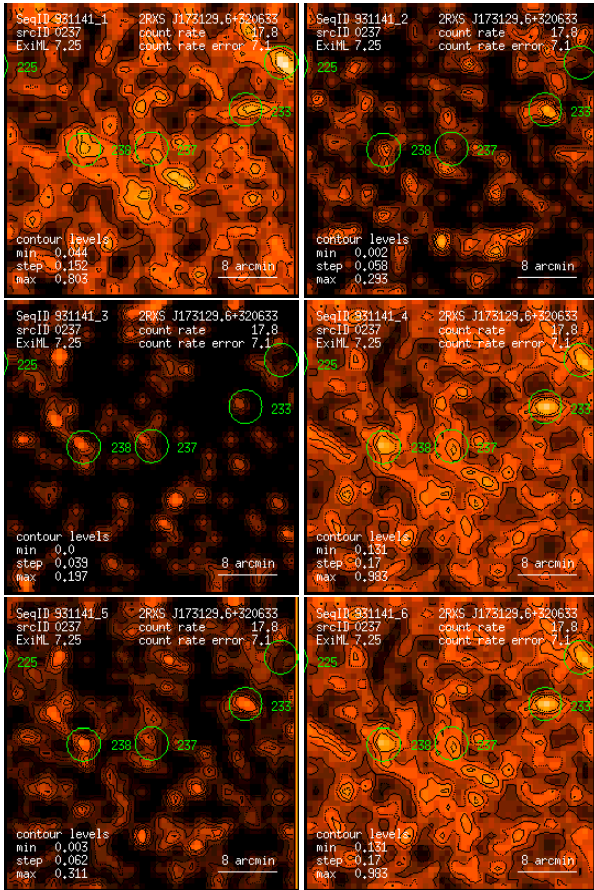
Figure 237: RASS 931141: detection 0237: band rate images, Gaussian filter: (1) PSPC channels 11 – 41, (2) 52 – 90, (3) 91 – 201, (4) 11 – 235, (5) 52 – 201, (6) 11 – 201. Broad band rates in counts/ks. Band rate contour levels in counts/ks/arcmin 2 .
