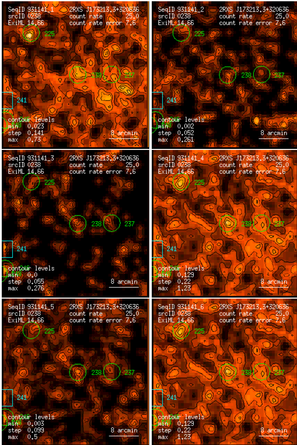
Figure 238: RASS 931141: detection 0238: band rate images, Gaussian filter: (1) PSPC channels 11 – 41, (2) 52 – 90, (3) 91 – 201, (4) 11 – 235, (5) 52 – 201, (6) 11 – 201. Broad band rates in counts/ks. Band rate contour levels in counts/ks/arcmin 2 .
