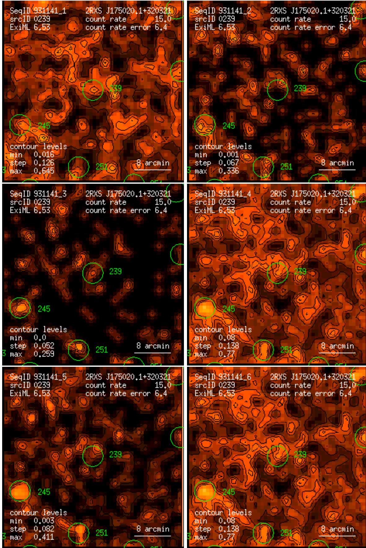
Figure 239: RASS 931141: detection 0239: band rate images, Gaussian filter: (1) PSPC channels 11 – 41, (2) 52 – 90, (3) 91 – 201, (4) 11 – 235, (5) 52 – 201, (6) 11 – 201. Broad band rates in counts/ks. Band rate contour levels in counts/ks/arcmin 2 .
