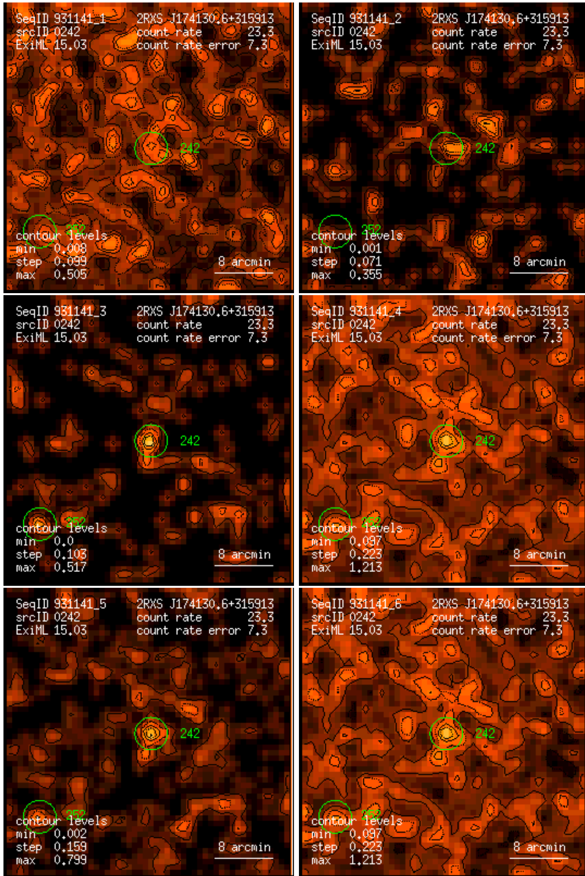
Figure 242: RASS 931141: detection 0242: band rate images, Gaussian filter: (1) PSPC channels 11 – 41, (2) 52 – 90, (3) 91 – 201, (4) 11 – 235, (5) 52 – 201, (6) 11 – 201. Broad band rates in counts/ks. Band rate contour levels in counts/ks/arcmin 2 .
