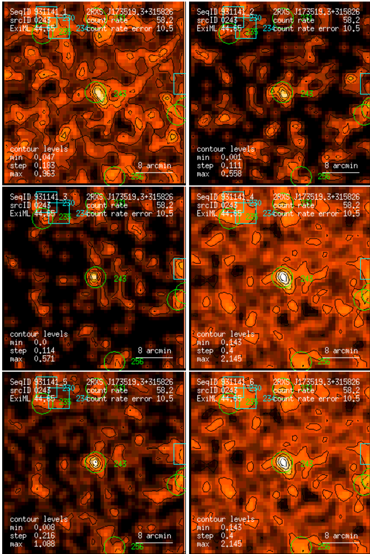
Figure 243: RASS 931141: detection 0243: band rate images, Gaussian filter: (1) PSPC channels 11 – 41, (2) 52 – 90, (3) 91 – 201, (4) 11 – 235, (5) 52 – 201, (6) 11 – 201. Broad band rates in counts/ks. Band rate contour levels in counts/ks/arcmin 2 .
