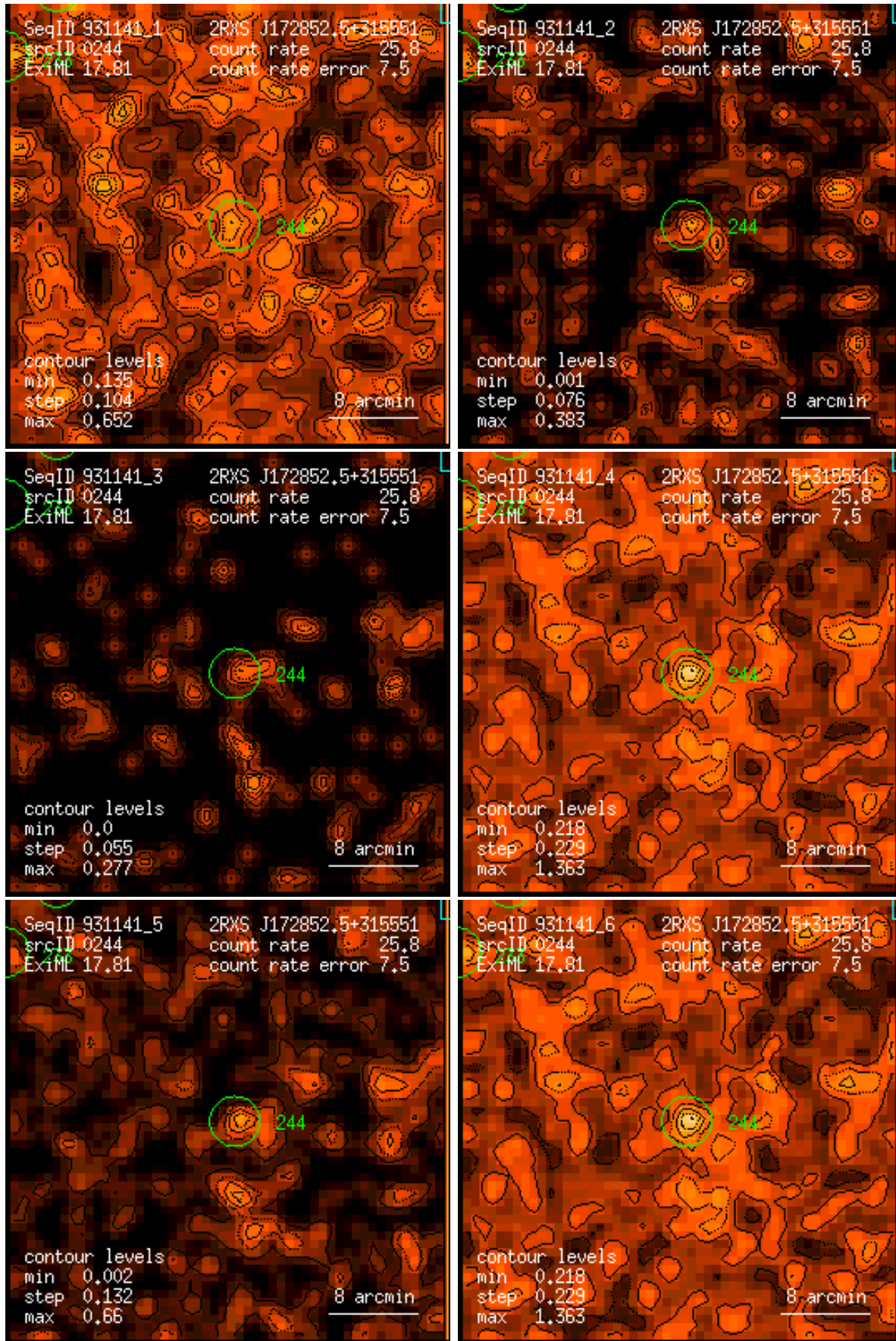
Figure 244: RASS 931141: detection 0244: band rate images, Gaussian filter: (1) PSPC channels 11 – 41, (2) 52 – 90, (3) 91 – 201, (4) 11 – 235, (5) 52 – 201, (6) 11 – 201. Broad band rates in counts/ks. Band rate contour levels in counts/ks/arcmin 2 .
