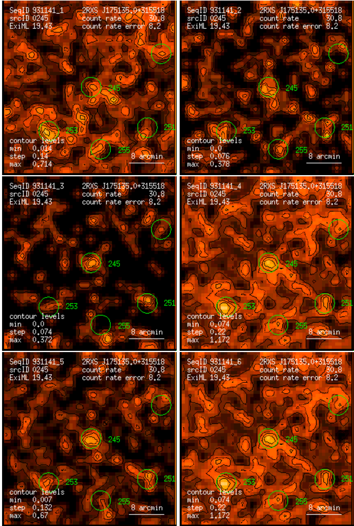
Figure 245: RASS 931141: detection 0245: band rate images, Gaussian filter: (1) PSPC channels 11 – 41, (2) 52 – 90, (3) 91 – 201, (4) 11 – 235, (5) 52 – 201, (6) 11 – 201. Broad band rates in counts/ks. Band rate contour levels in counts/ks/arcmin 2 .
