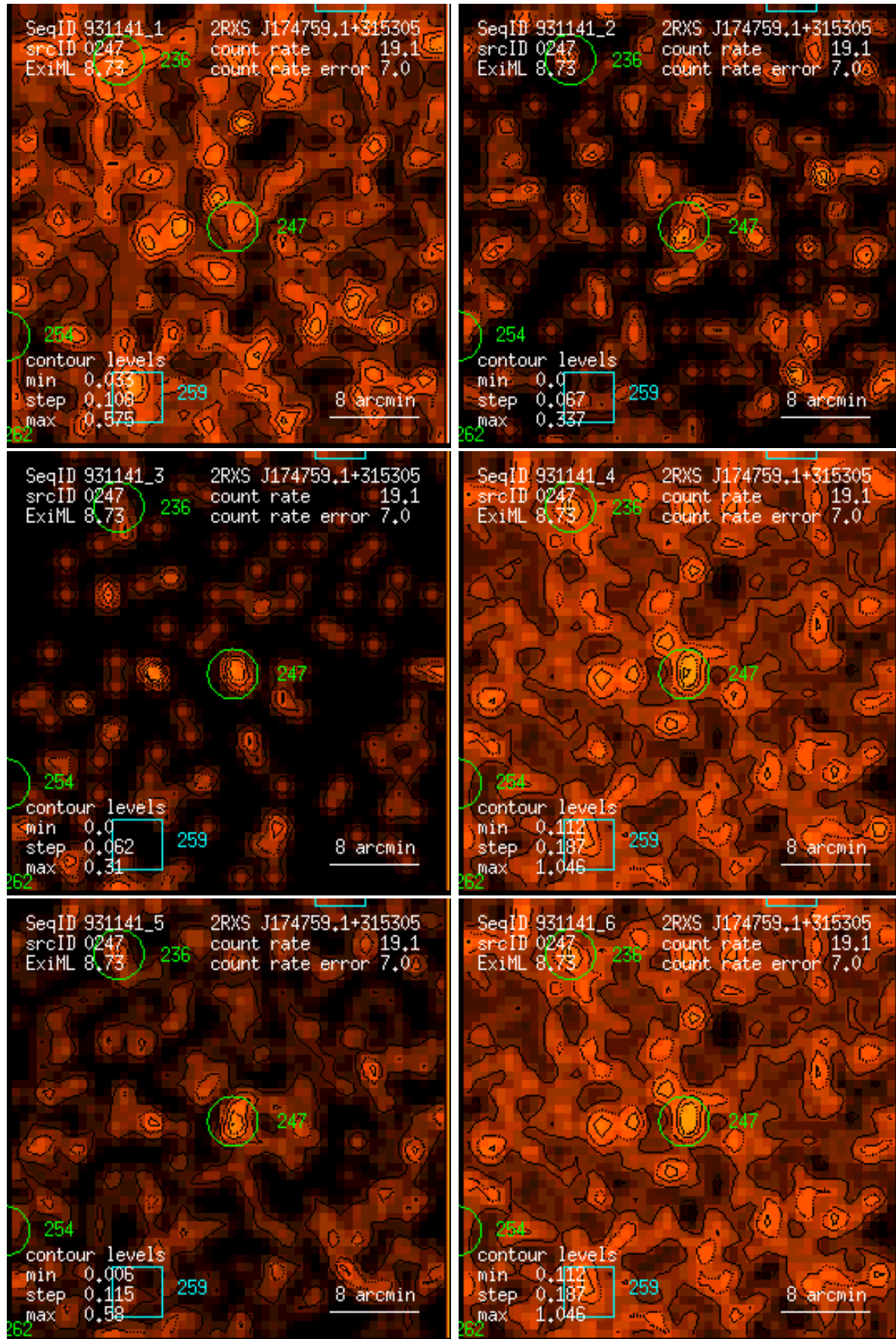
Figure 247: RASS 931141: detection 0247: band rate images, Gaussian filter: (1) PSPC channels 11 – 41, (2) 52 – 90, (3) 91 – 201, (4) 11 – 235, (5) 52 – 201, (6) 11 – 201. Broad band rates in counts/ks. Band rate contour levels in counts/ks/arcmin 2 .
