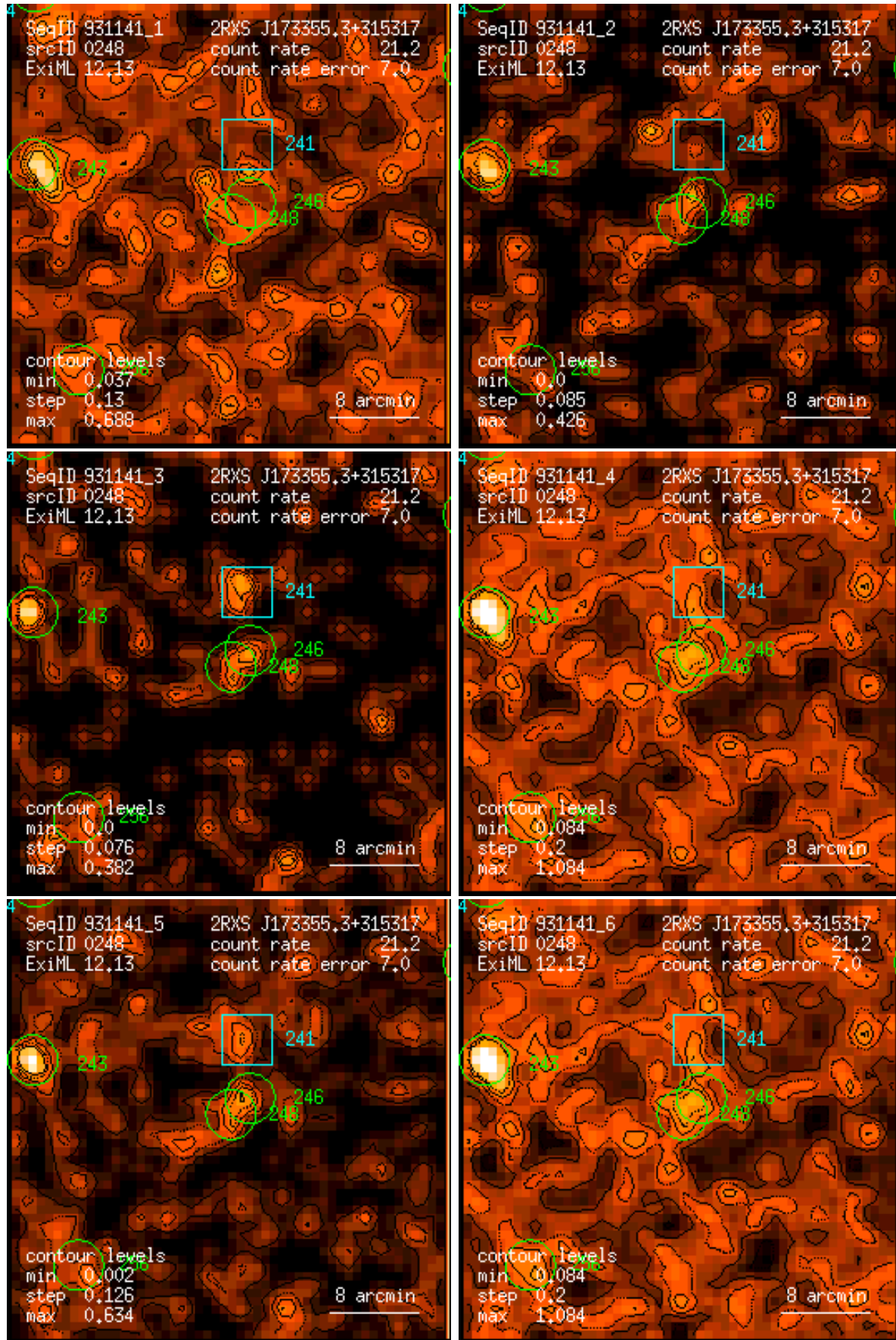
Figure 248: RASS 931141: detection 0248: band rate images, Gaussian filter: (1) PSPC channels 11 – 41, (2) 52 – 90, (3) 91 – 201, (4) 11 – 235, (5) 52 – 201, (6) 11 – 201. Broad band rates in counts/ks. Band rate contour levels in counts/ks/arcmin 2 .
