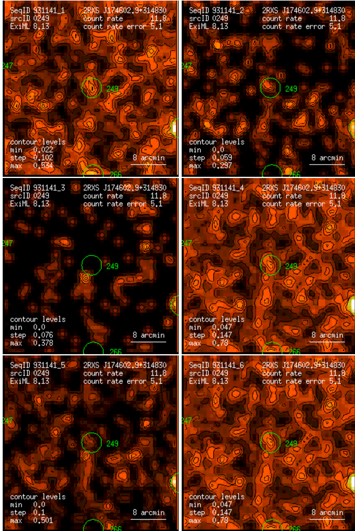
Figure 249: RASS 931141: detection 0249: band rate images, Gaussian filter: (1) PSPC channels 11 – 41, (2) 52 – 90, (3) 91 – 201, (4) 11 – 235, (5) 52 – 201, (6) 11 – 201. Broad band rates in counts/ks. Band rate contour levels in counts/ks/arcmin 2 .
