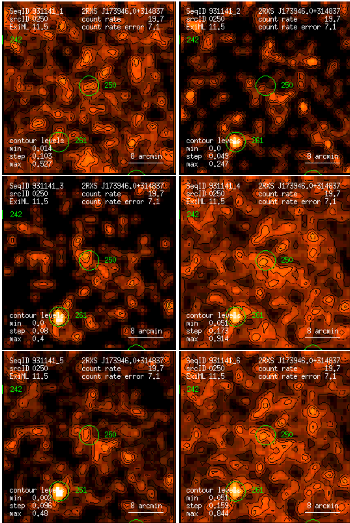
Figure 250: RASS 931141: detection 0250: band rate images, Gaussian filter: (1) PSPC channels 11 – 41, (2) 52 – 90, (3) 91 – 201, (4) 11 – 235, (5) 52 – 201, (6) 11 – 201. Broad band rates in counts/ks. Band rate contour levels in counts/ks/arcmin 2 .
