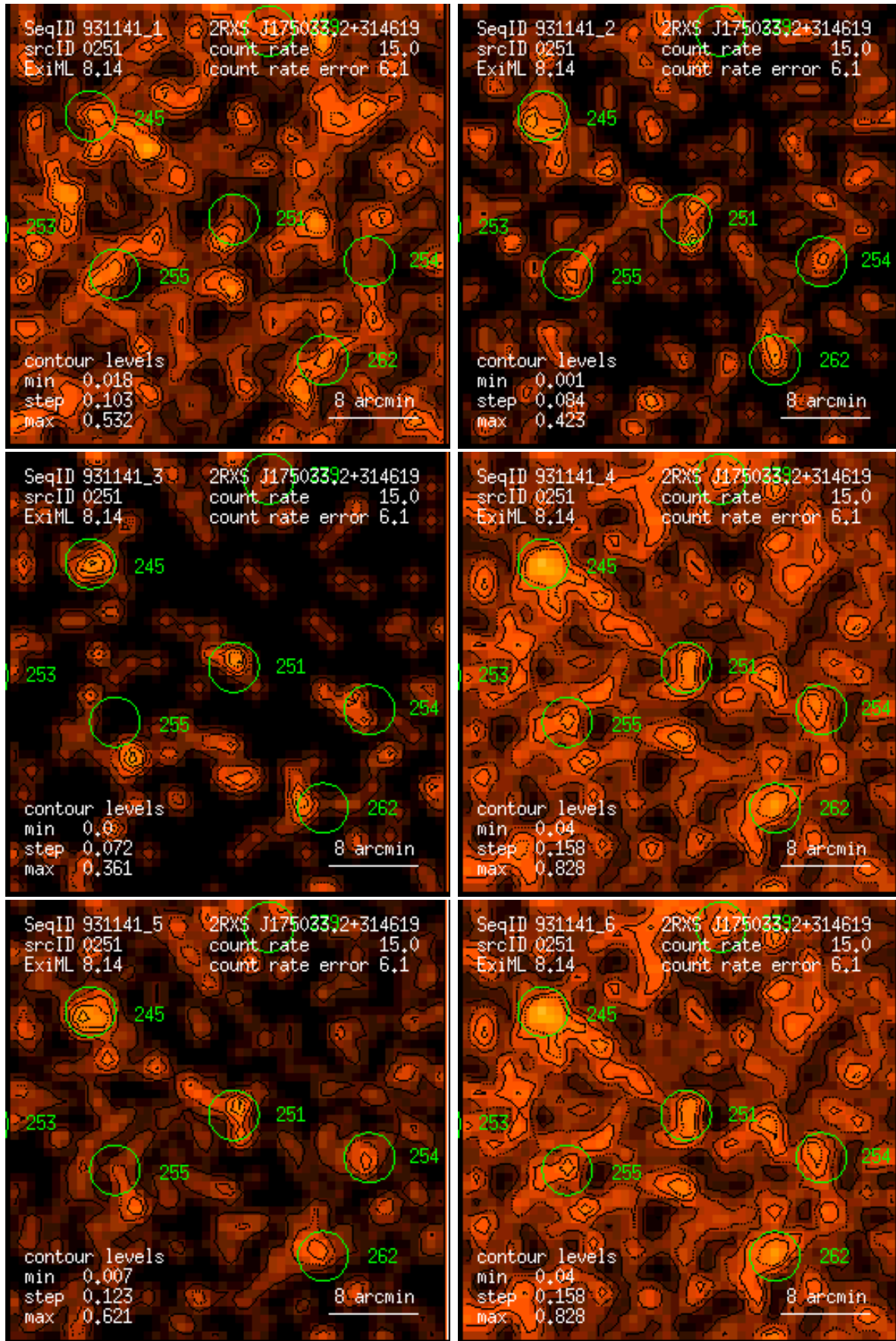
Figure 251: RASS 931141: detection 0251: band rate images, Gaussian filter: (1) PSPC channels 11 – 41, (2) 52 – 90, (3) 91 – 201, (4) 11 – 235, (5) 52 – 201, (6) 11 – 201. Broad band rates in counts/ks. Band rate contour levels in counts/ks/arcmin 2 .
