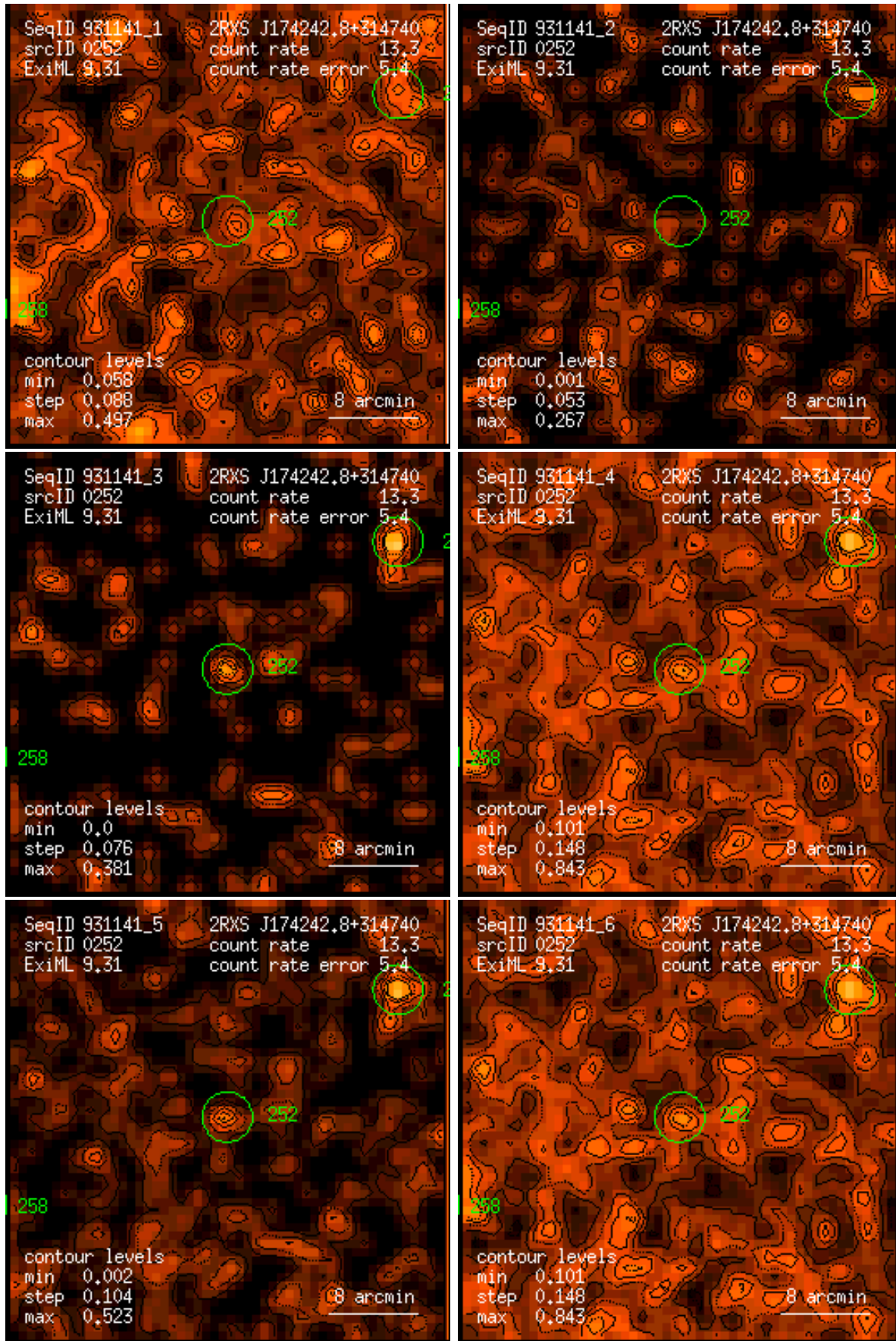
Figure 252: RASS 931141: detection 0252: band rate images, Gaussian filter: (1) PSPC channels 11 – 41, (2) 52 – 90, (3) 91 – 201, (4) 11 – 235, (5) 52 – 201, (6) 11 – 201. Broad band rates in counts/ks. Band rate contour levels in counts/ks/arcmin 2 .
