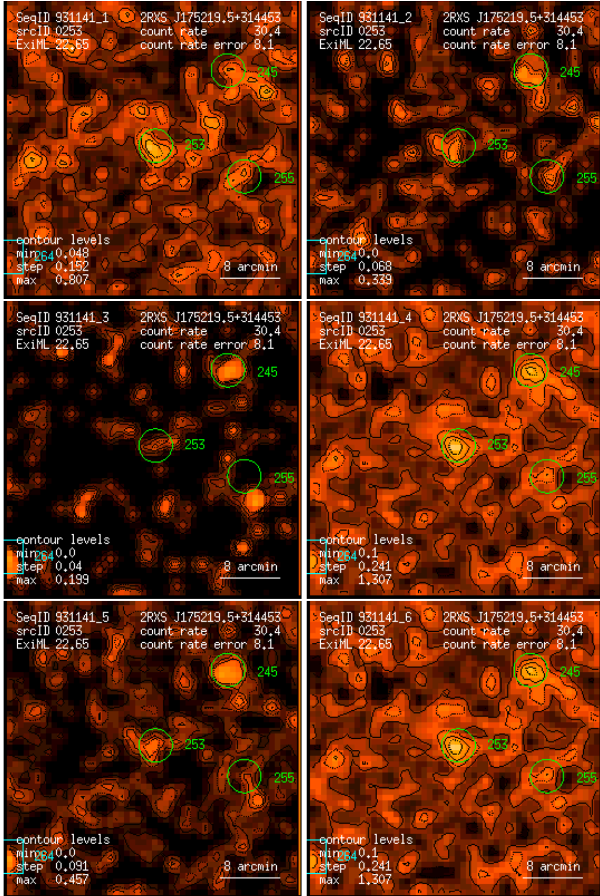
Figure 253: RASS 931141: detection 0253: band rate images, Gaussian filter: (1) PSPC channels 11 – 41, (2) 52 – 90, (3) 91 – 201, (4) 11 – 235, (5) 52 – 201, (6) 11 – 201. Broad band rates in counts/ks. Band rate contour levels in counts/ks/arcmin 2 .
