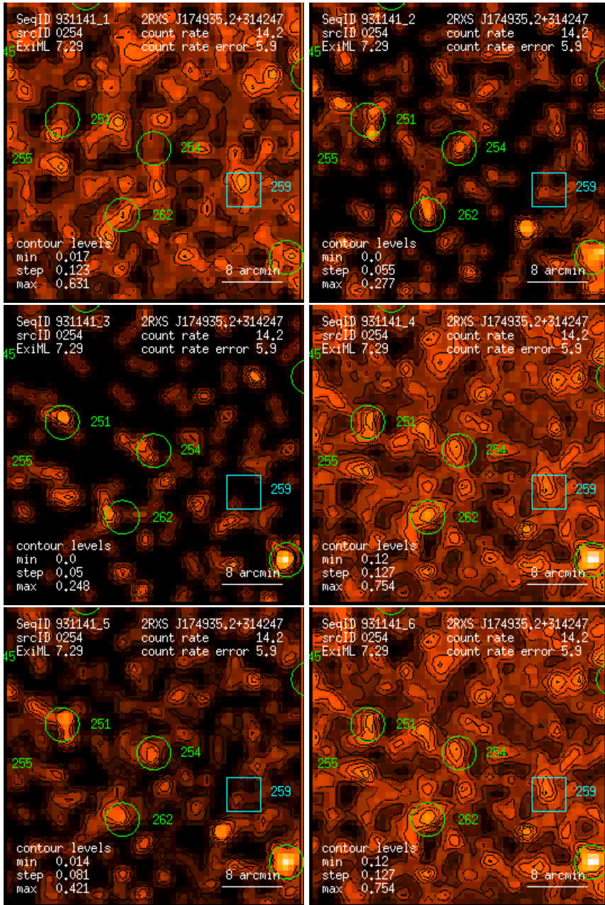
Figure 254: RASS 931141: detection 0254: band rate images, Gaussian filter: (1) PSPC channels 11 – 41, (2) 52 – 90, (3) 91 – 201, (4) 11 – 235, (5) 52 – 201, (6) 11 – 201. Broad band rates in counts/ks. Band rate contour levels in counts/ks/arcmin 2 .
